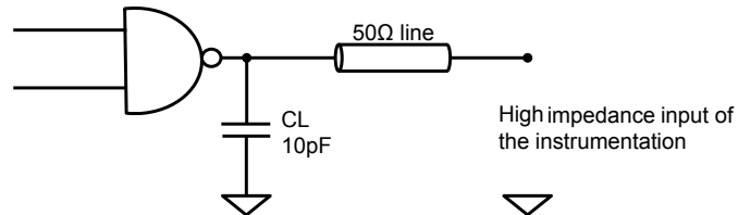
Figure 3. Test configuration
