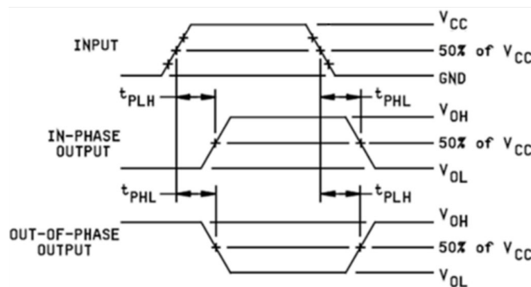
Figure 4. Timings
