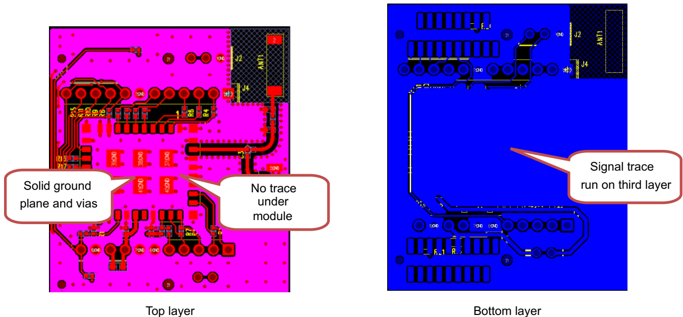
Figure 11. Module Layout
