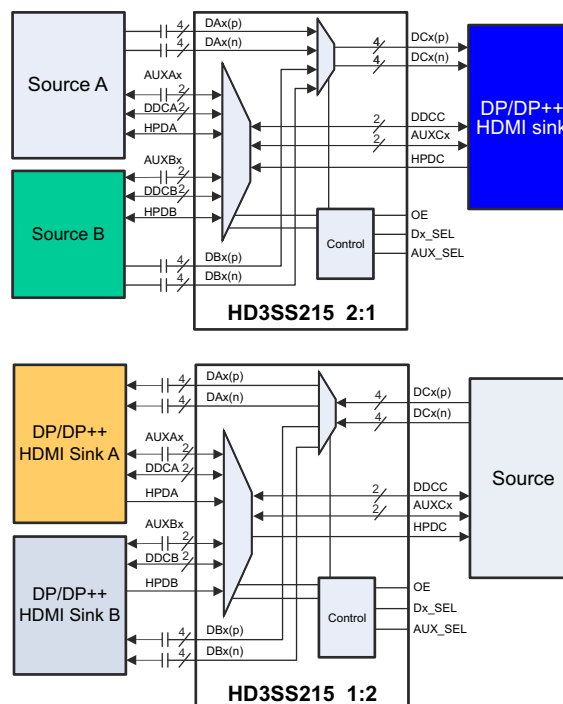
Application Schematic
