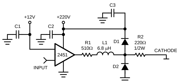
Figure 13. One Channel of the LM2451 with the Recommended Application Circuit
