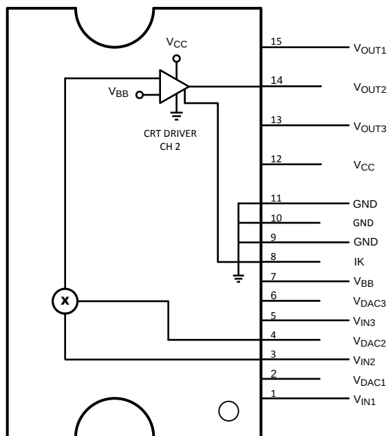
Figure 1. Top View
