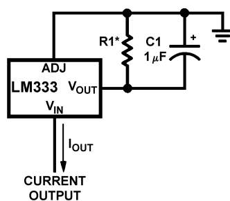
Figure 6. High-Performance 9-Ampere Adjustable Regulator
