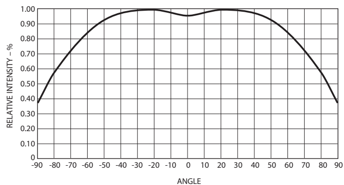
Figure 10: Relative Intensity vs. Angle for HSMx-C150/C170/C190/C191/C265
