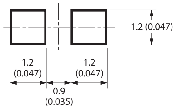
Figure 14: Recommended Soldering Pattern for HSMx-C170/C177
