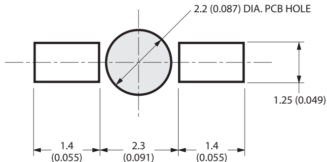
Figure 18: Recommended Soldering Pattern for HSMx-C265
