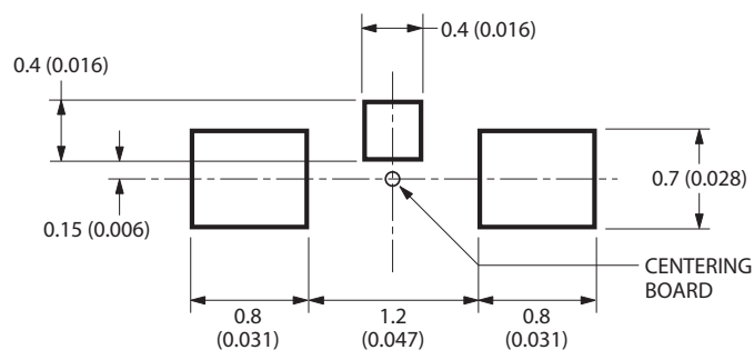
Figure 17: Recommended Soldering Pattern for HSMx-C120
