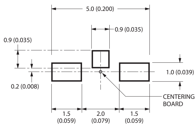
Figure 18: Recommended Soldering Pattern for HSMx-C265
