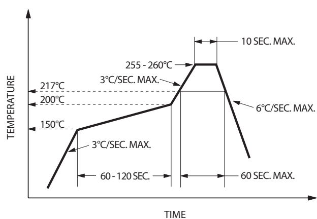
Figure 12: Recommended Lead-Free Reflow Soldering Profile
