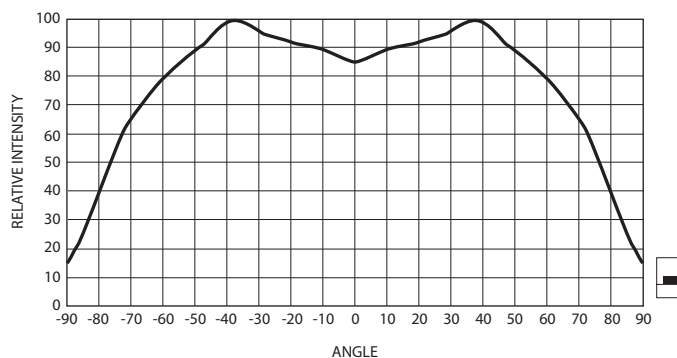
Figure 8: Relative Intensity vs. Angle for HSMx-C120
