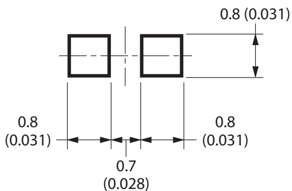
Figure 15: Recommended Soldering Pattern for HSMx-C190/C191/C197
