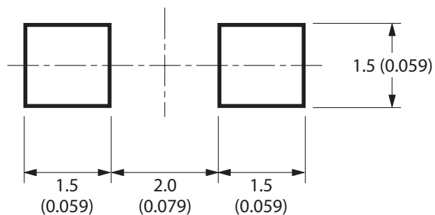
Figure 13: Recommended Soldering Pattern for HSMx-C150
