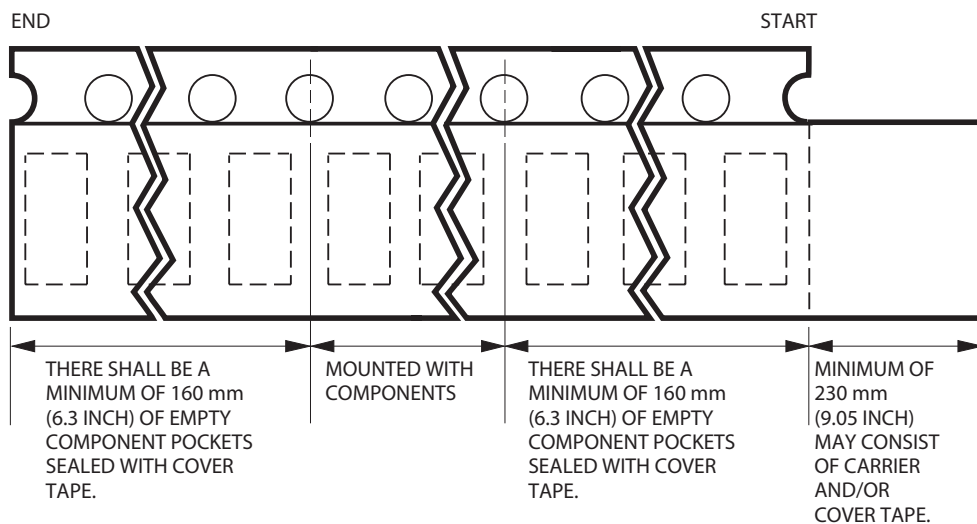
Figure 22: Tape Leader and Trailer Dimensions
