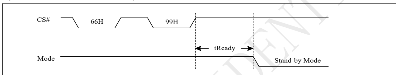
Figure 10-50a Reset Sequence
