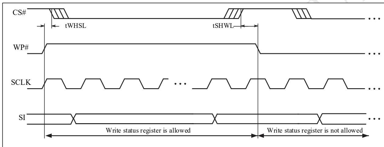
Figure 5-7 WP Timing
