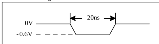
Figure 5-2 Input Test Waveforms and Measurement Level
