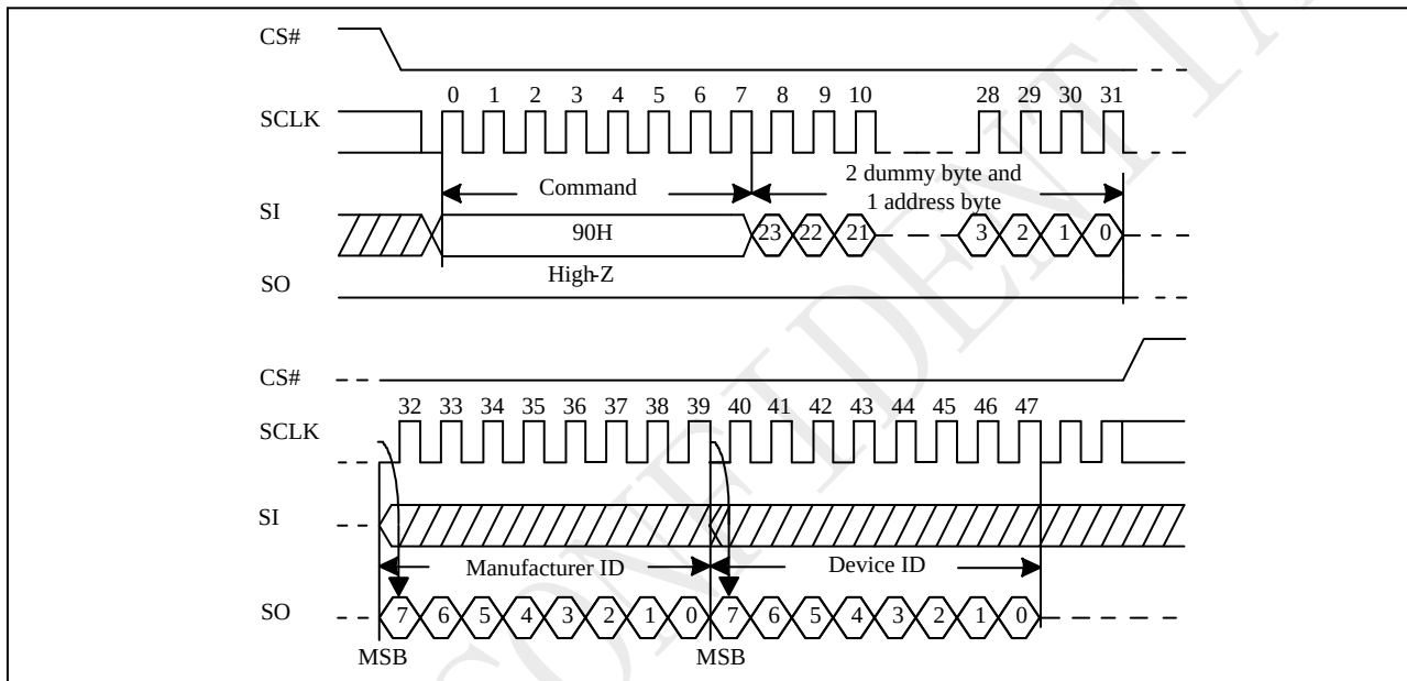
Figure 10-41 Read Electronic Manufacturer & Device ID (REMS) Sequence (Command 90)
