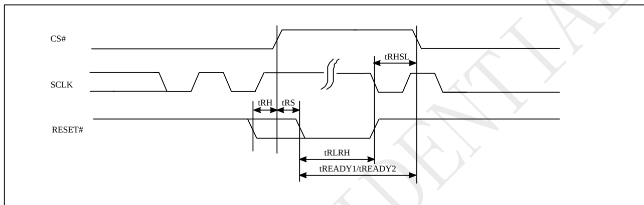
Figure 10-56 RESET Timing
