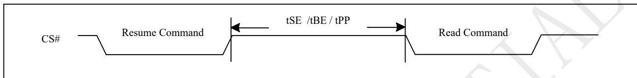
Figure 9-60a Resume to Read Latency (QPI)
