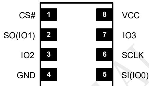
8-Pad WSON8(6x5/8x6mm)
