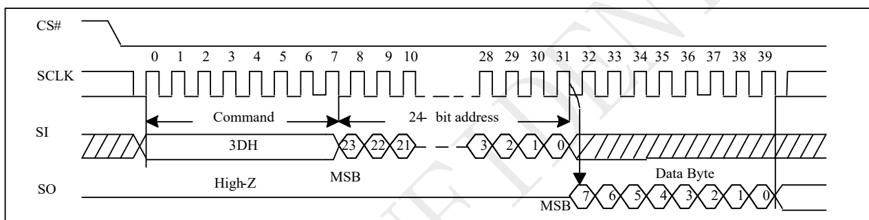
Figure 9-64 Read Block Lock Status (SPI)
