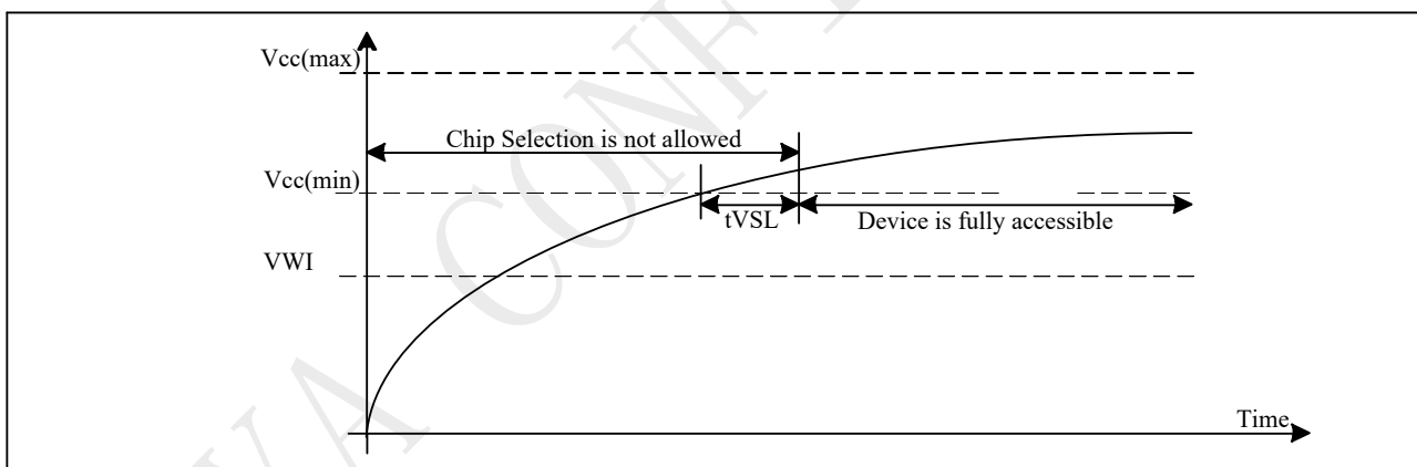
Figure 5-9 Power-up Timing
