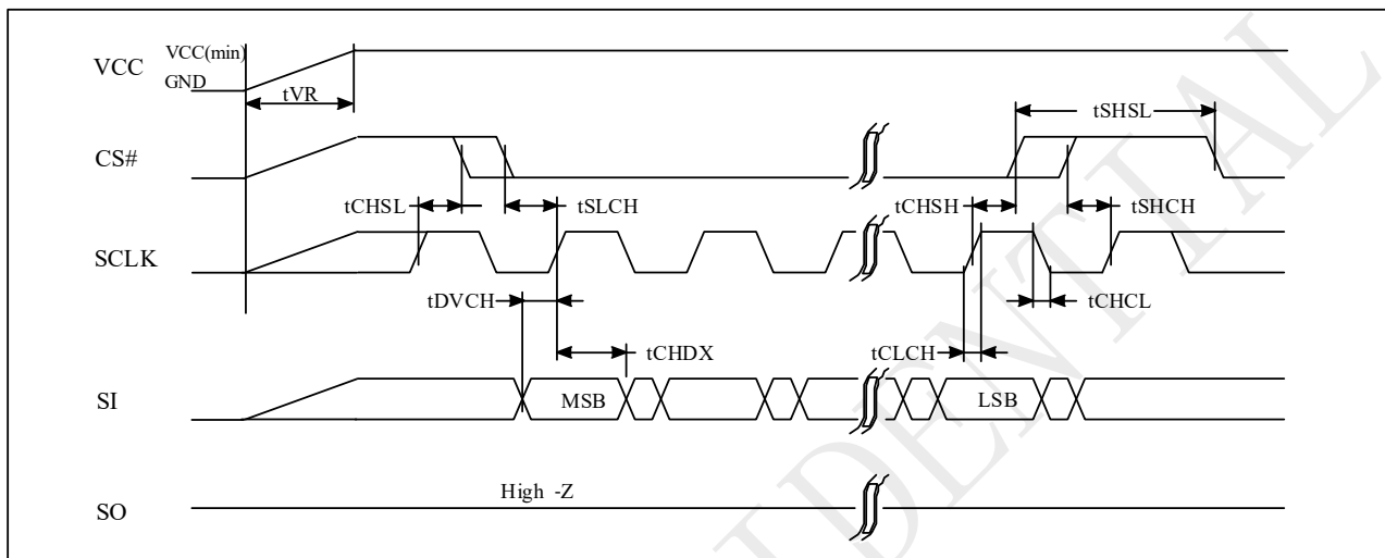
Figure 5-9 Power-up Timing
