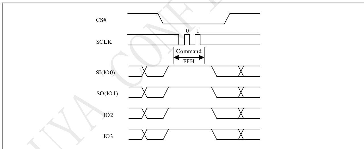
Figure 9-35 Disable QPI Sequence (QPI)
