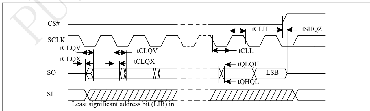
Figure 5-5 Output Timing
