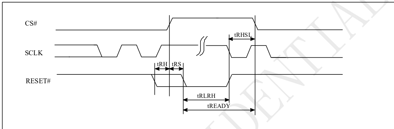
Figure 9-68 RESET Timing
