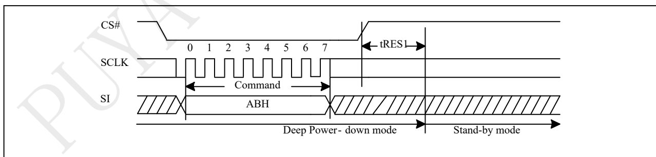
Figure 9-48a Release from Deep Power-down (RDP) Sequence (SPI)
