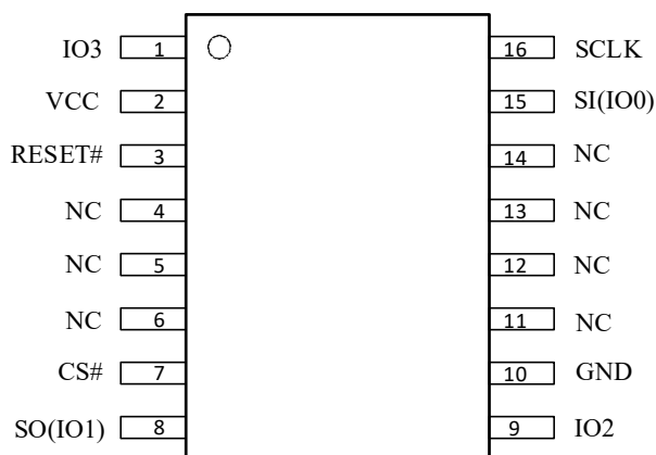
Figure 3-3 for SOP16 package
