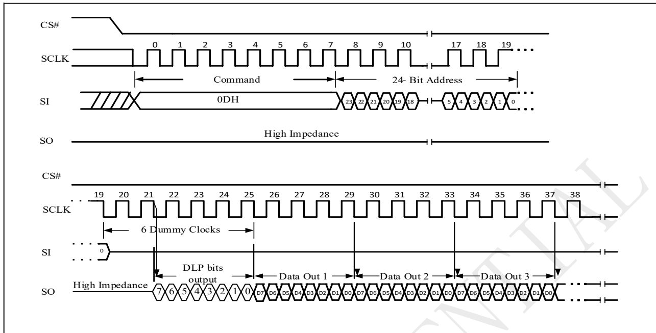
Figure 9-30e DTR 1IO Read with DLP bits output Sequence (SPI)
