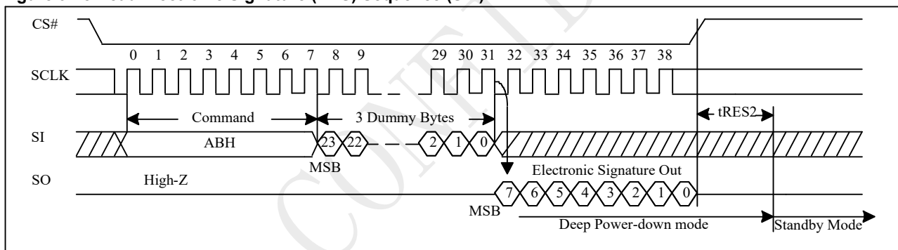
Figure 9-48 Read Electronic Signature (RES) Sequence (SPI)
