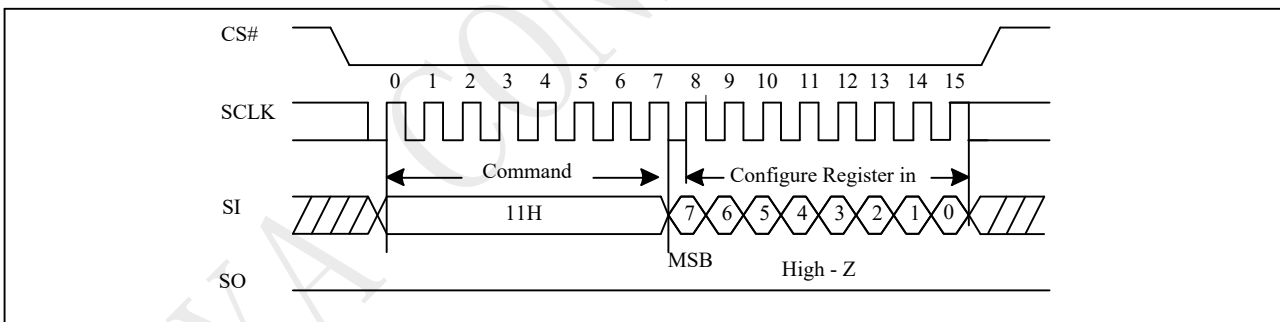
Figure 9-8 Write Configure Register (WRCR) Sequence (SPI)
