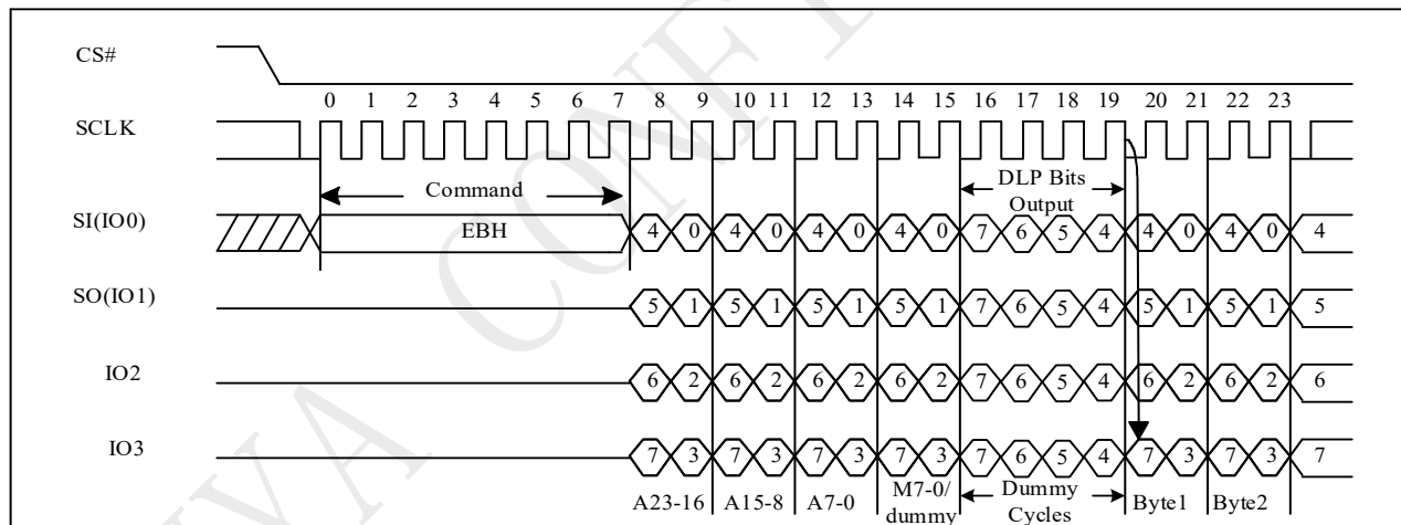
Figure 9-30d 4IO Read with DLP bits output Sequence (SPI)
