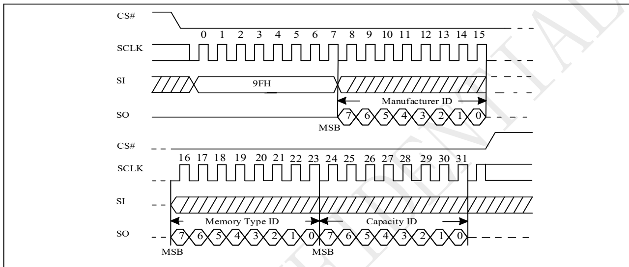
Figure 9-57a Read Identification (RDID) Sequence (QPI)
