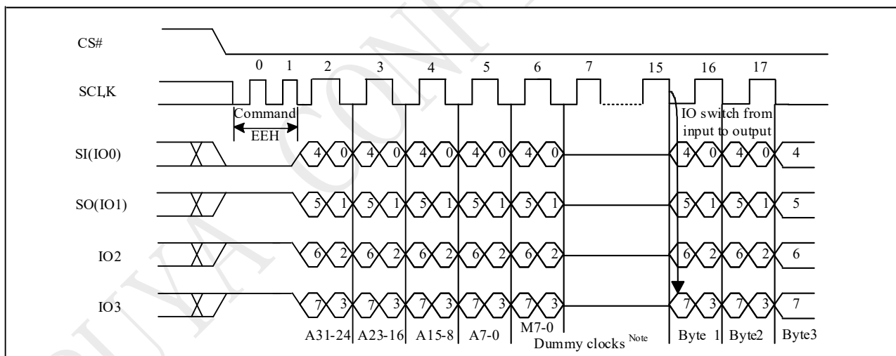
Figure 9-28a DTR 4IO Read with 4-Byte Address Sequence (QPI, M5-4 ≠ (1,0))
