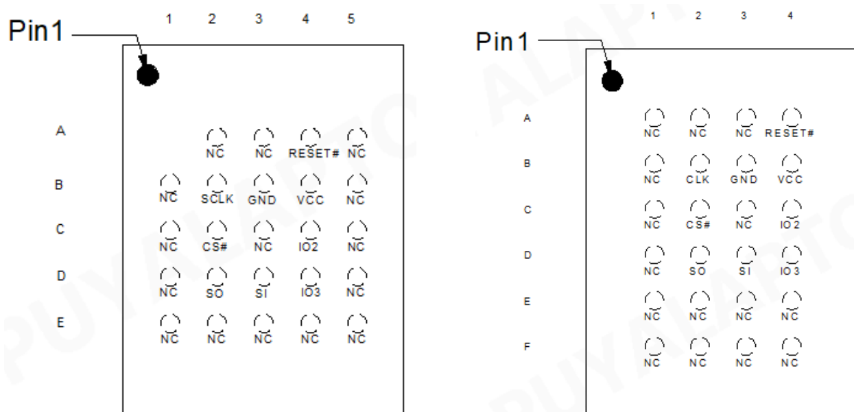
24-Ball TFBGA (5x5 Array) –TF
