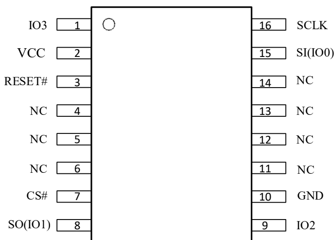
Figure 3-2 for SOP16 package
