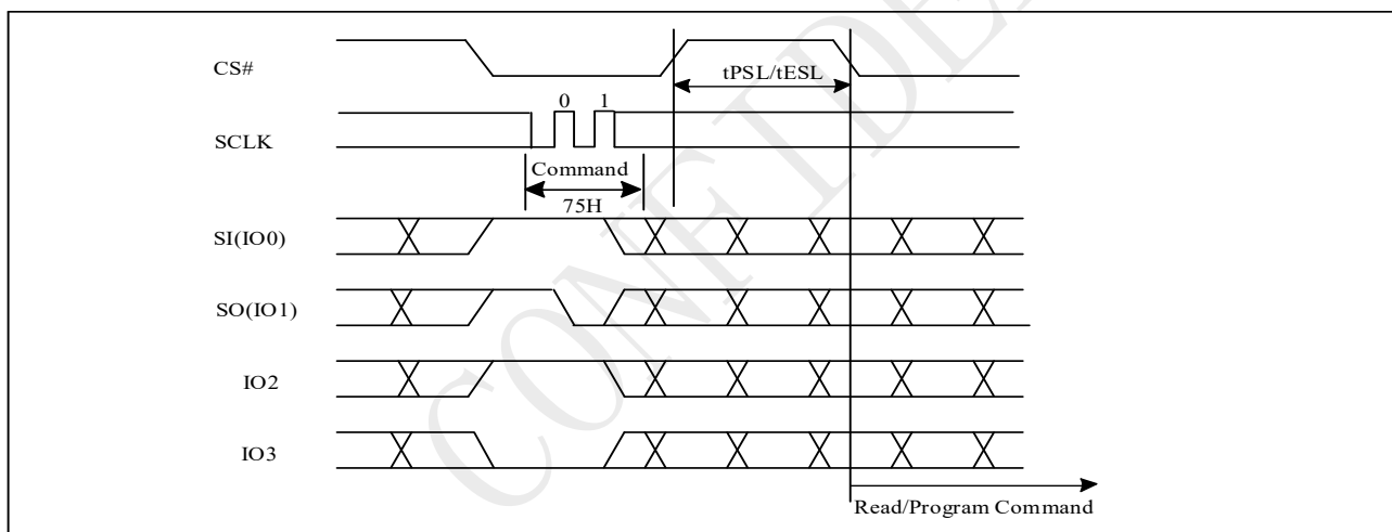
Figure 9-59a Suspend to Read/Program Latency(QPI)
