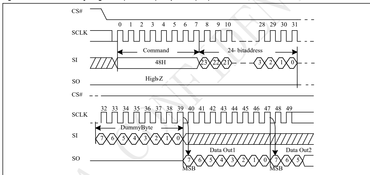
Figure 9-51 Read Security Registers (RDSCUR) Sequence (SPI)
