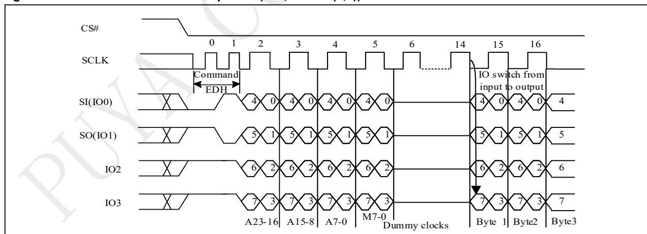
Figure 9-27b DTR 4IO Read Mode Sequence (QPI, M5-4 \neq (1,0))
