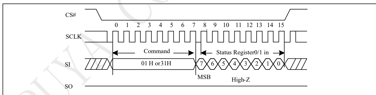
Figure 9-7 Write Status Register (WRSR) Sequence (SPI)
