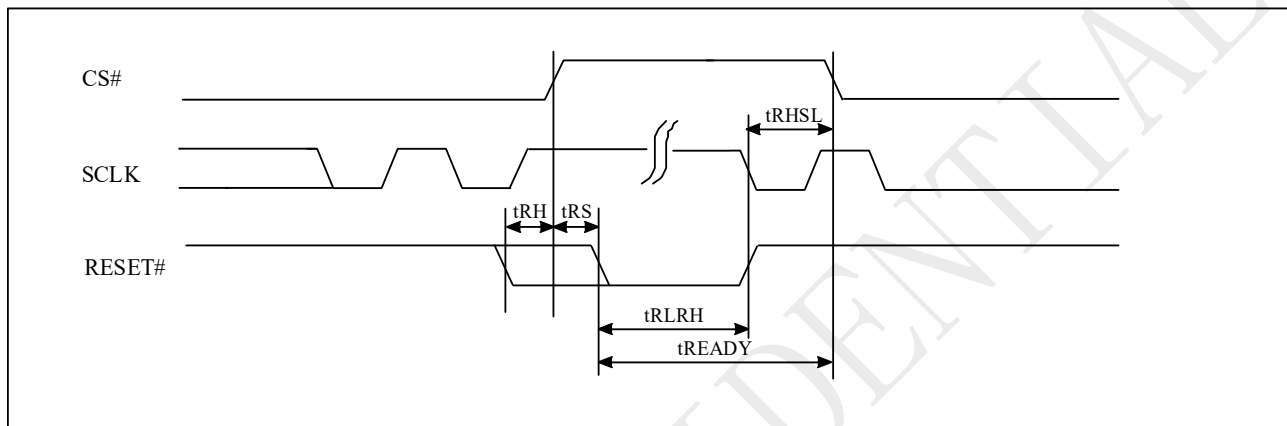
Figure 9-68 RESET Timing
