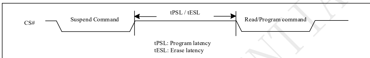
Figure 9-59a Suspend to Read/Program Latency(QPI)
