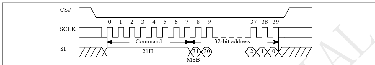
Figure 9-37 Sector Erase with 4-Byte Address Sequence (SPI)
