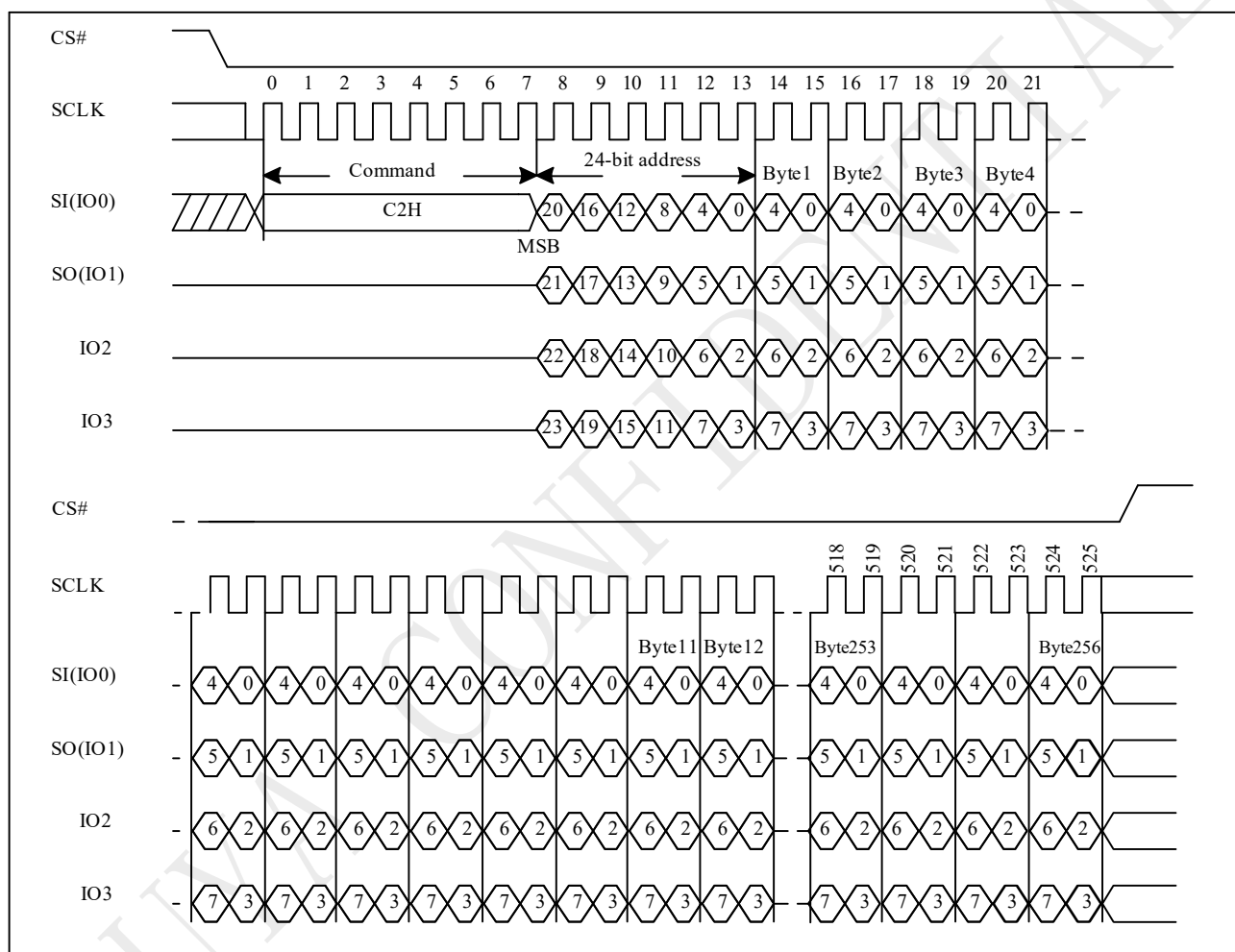
Figure 9-47 Quad Page Program (QPP) Sequence (SPI)
