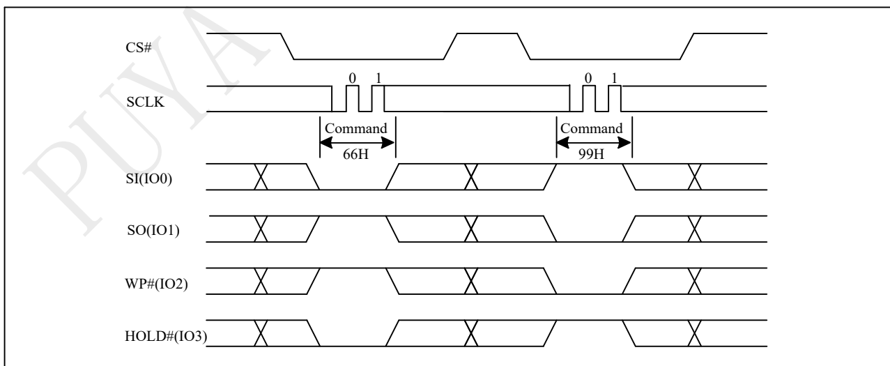
Figure 10-57b Reset Sequence(QPI)
