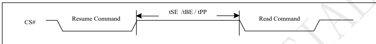
Figure 10-51a Resume to Read Latency(QPI)
