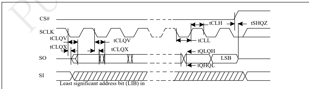
Figure 5-5 Output Timing
