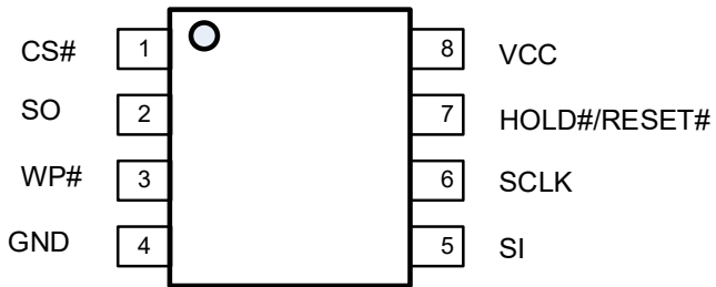
8-Lead SOP (208mil)
