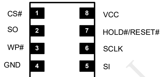
8-Pad WSON (6x5mm)
