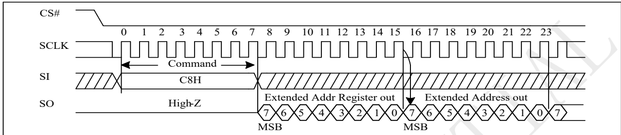
Figure 10-9 Read Extended Address Register Sequence (Command C8)
