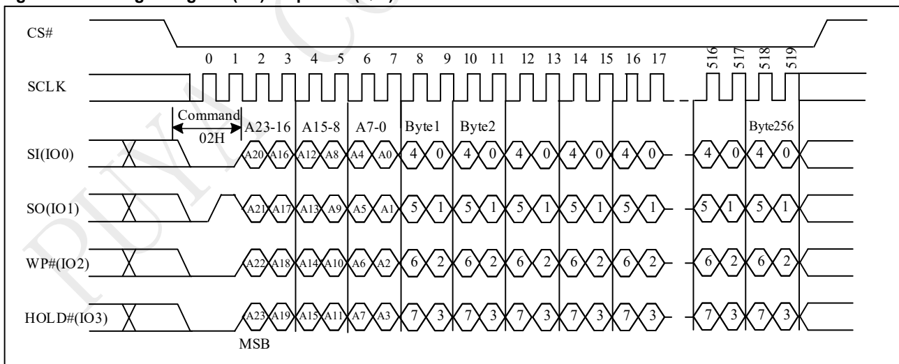
Figure 10-33a Page Program (PP) Sequence (QPI)
