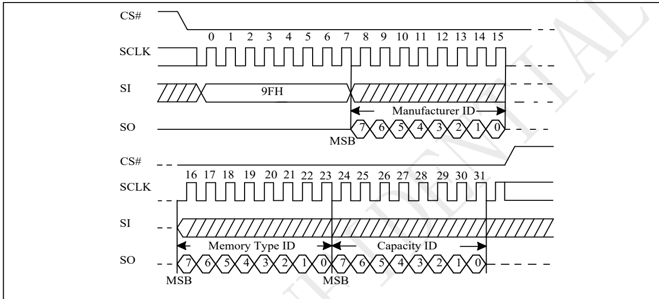
Figure 10-48a Read Identification (RDID) Sequence (QPI)
