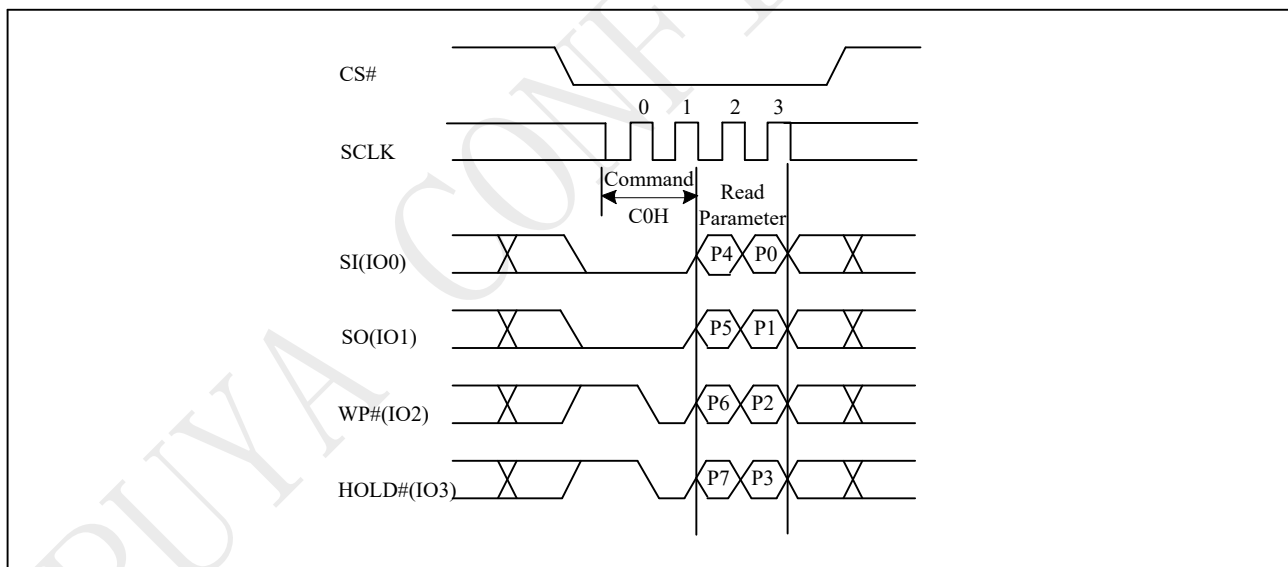
Figure 10-22 Set Read Parameters Sequence ( QPI )
