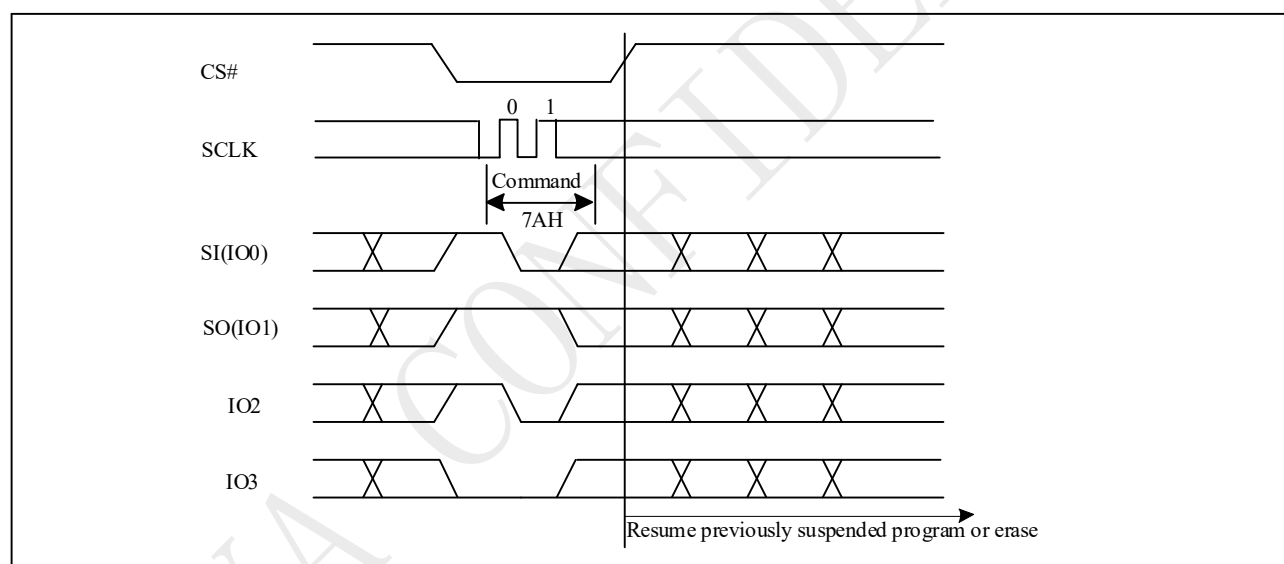
Figure 9-60a Resume to Read Latency (QPI)
