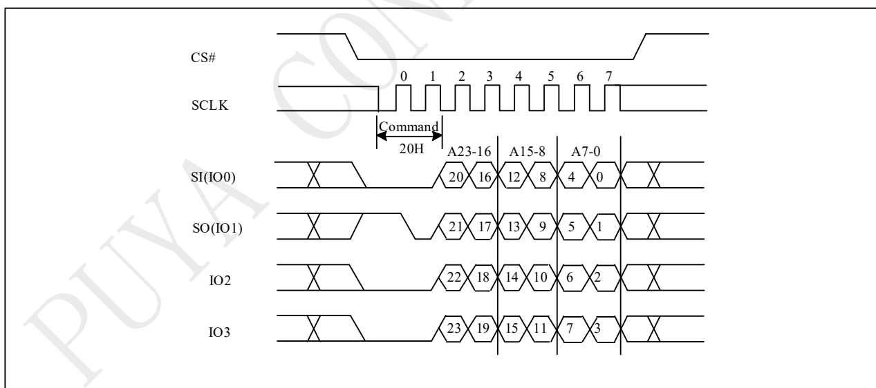
Figure 9-36a Sector Erase (SE) Sequence (QPI)
