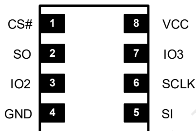
8-Pad WSON (6x5mm/8x6mm)
