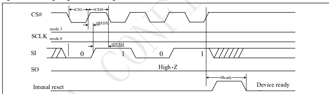
Figure 9-69 Timing Diagram and Timing Parameters
