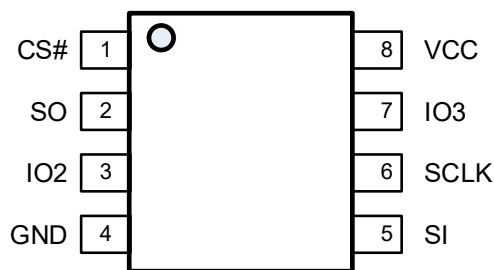
8-Lead SOP (208mil)
