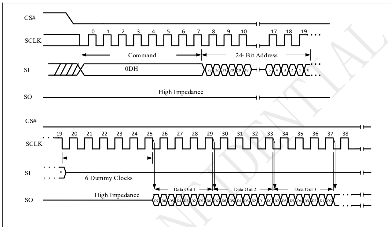
Figure 9-16 DTR Fast Read Sequence (Command 0D)
