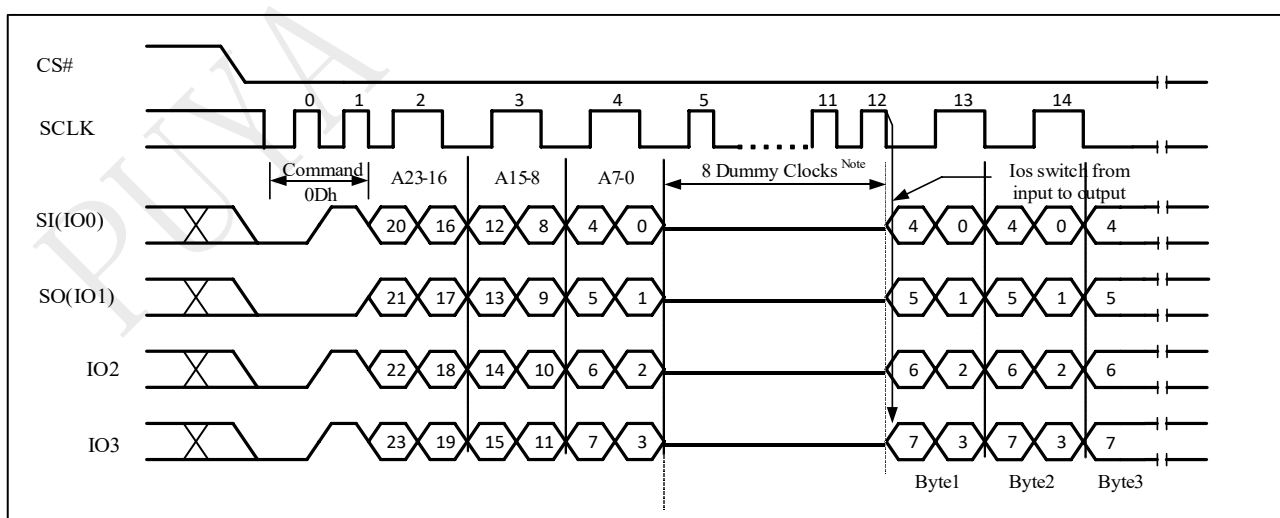
Figure 9-16a DTR Fast Read Sequence (QPI)
