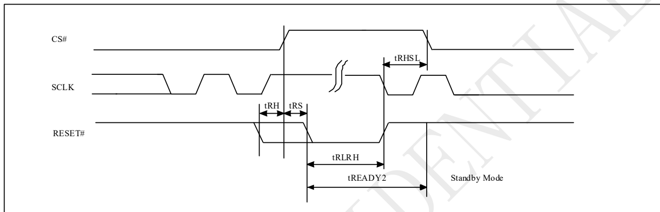
Figure 9-68 RESET Timing
