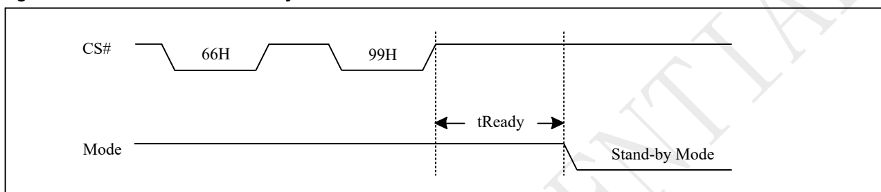
Figure 9-67a Reset Sequence
