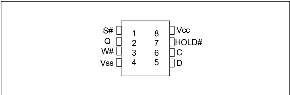
PDIP8/SOP8 (150mil/208mil)/TSSOP8/MSOP8/DFN8/UDFN8
