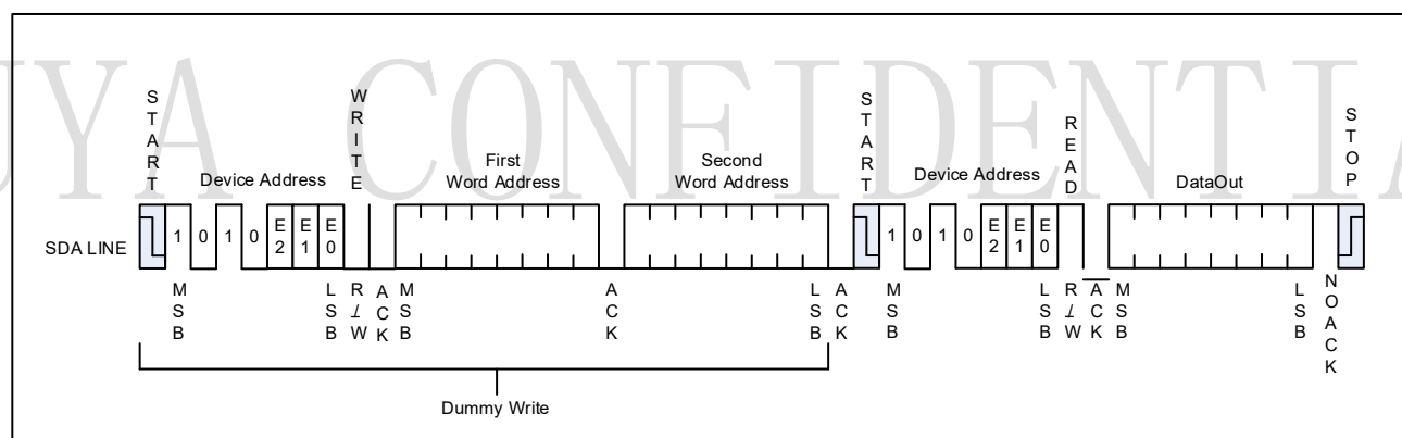
Figure 5-4 Random Read
