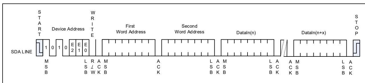
Figure 5-2 Page Write
