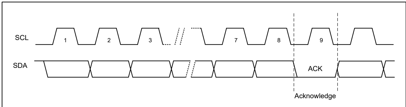
Figure 4-3 Output Acknowledge
