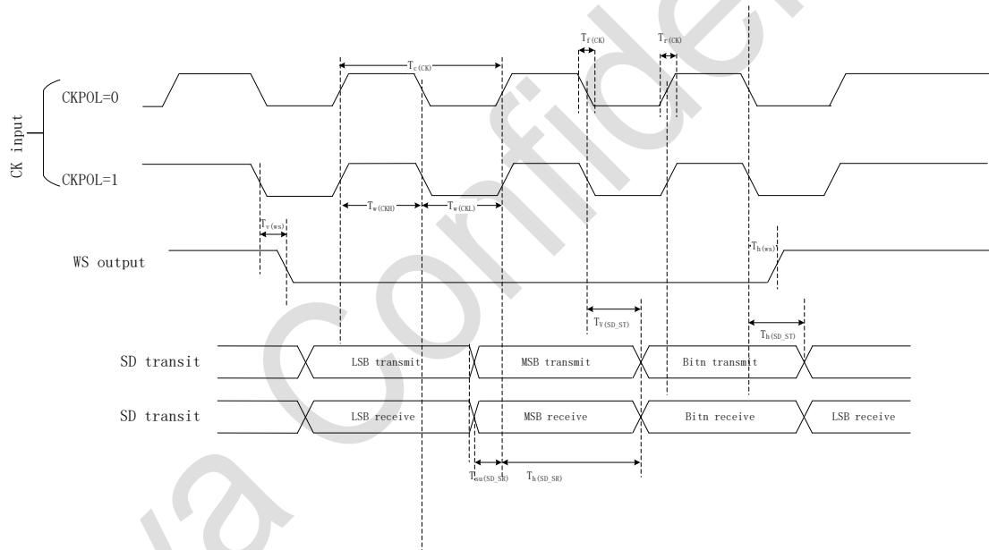
Figure 5-8 I²S timing diagram-Master mode(Philips protocol)
