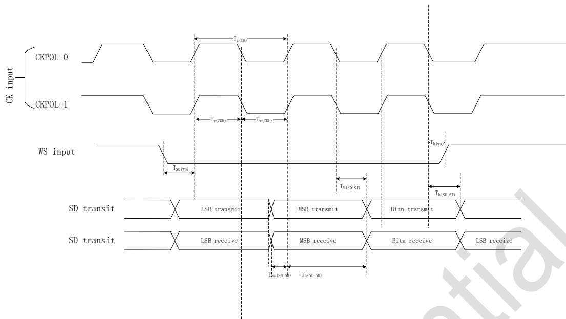
Figure 5-7 I²S timing diagram-Slave mode(Philips protocol)
