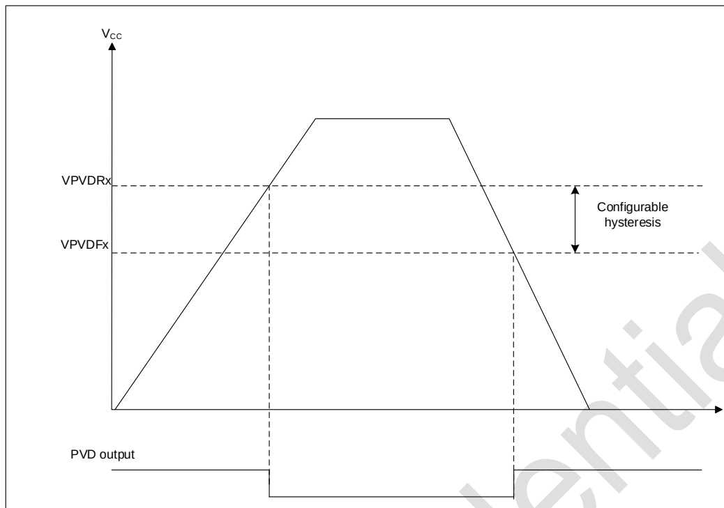
Figure 2-4 PVD threshold
