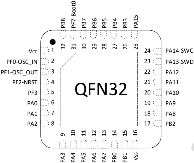
Figure 3-7 QFN32(4*4) Pinout2 PY32F031K2xUx (Top view)
