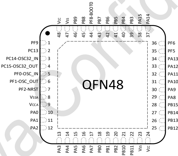
Figure 3-6 QFN48 PY32F071C1xU6 Pinout1(Top view)
