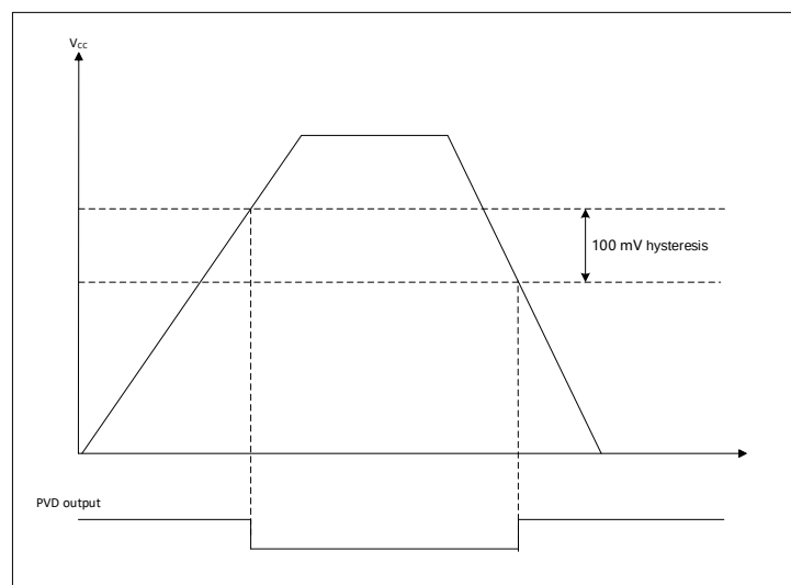
Figure 2-4 PVD threshold
