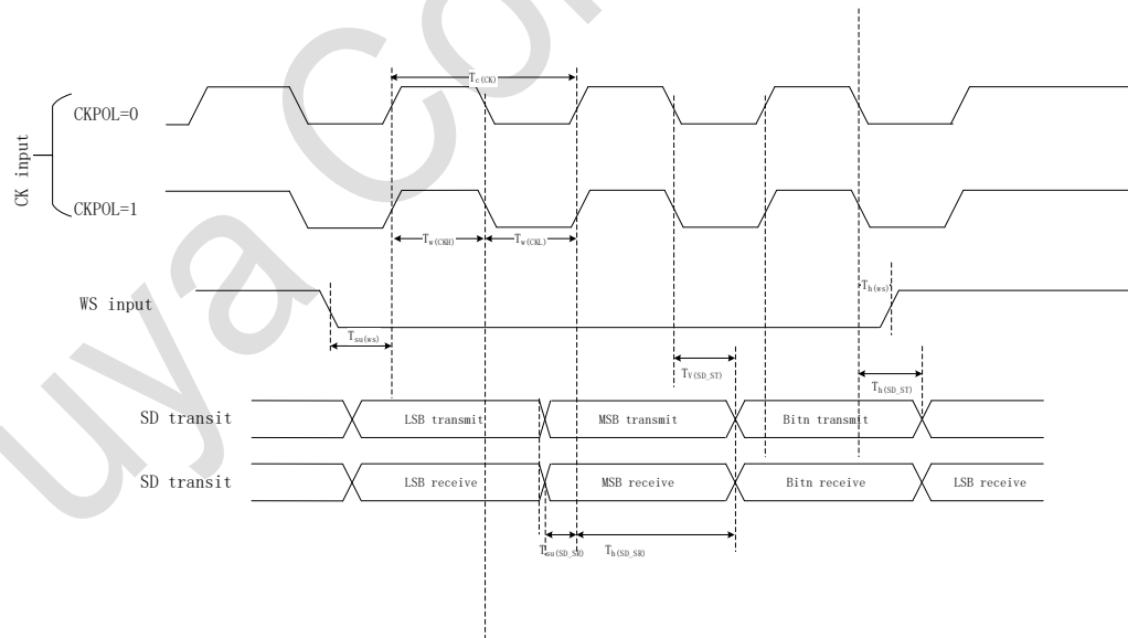
Figure 5-8 I 2 S slave timing diagram (Philips protocol)
