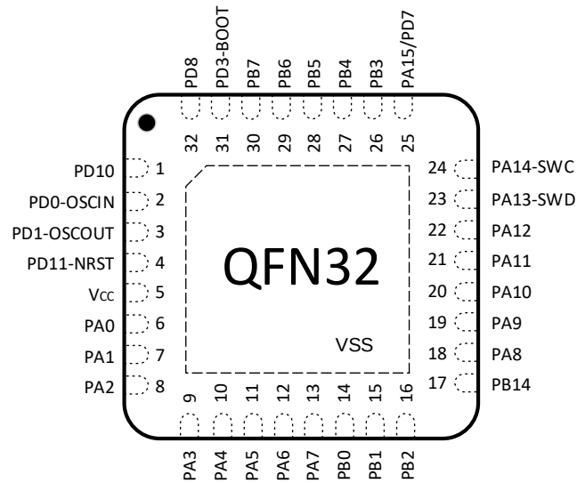
Figure 3-5 QFN32 (4 * 4) PY32F410K1xU7 Pinout1 (Top view)
