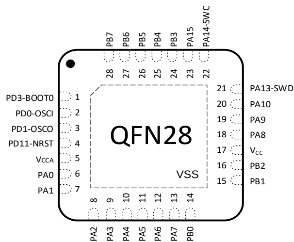
Figure 3-6 QFN28 (4*4) PY32F410G1xU7 Pinout1 (Top view)
