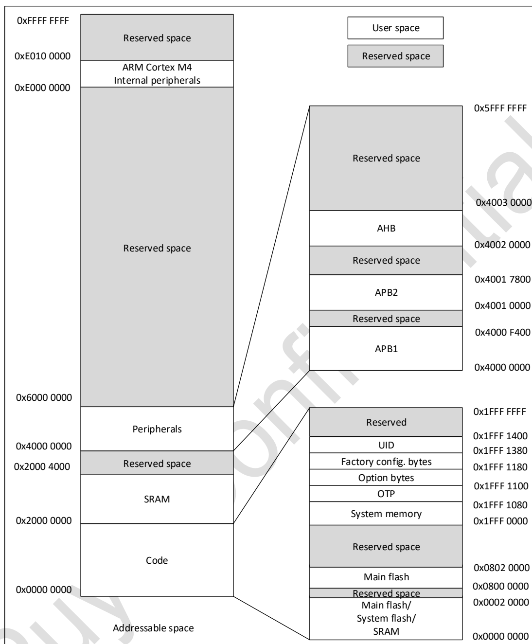
Figure 4-1 Memory mapping
