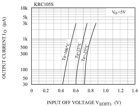
Fig 11. I_O vs. V_{I(OFF)}
