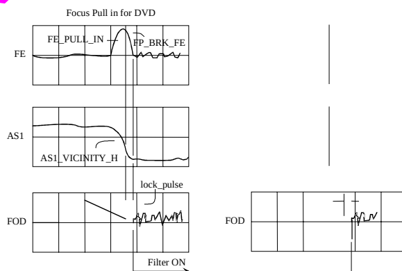
Figure 9 Focus Pull In (With Parameter Bit 0 Set and Bit 2 Cleared)
