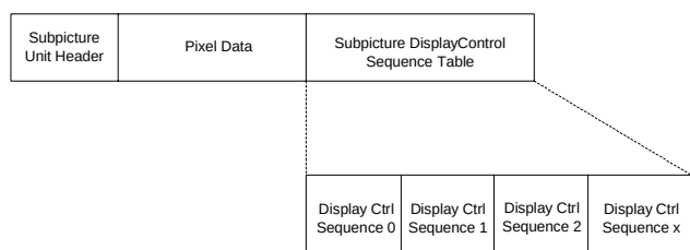
Figure 24 Typical Subpicture Data Framing Format
