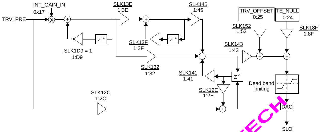
Figure 11 Sled Track Following Equalizer
