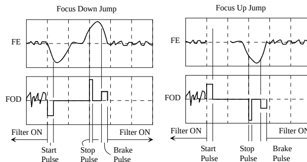
Figure 19 Focus Up and Down Jump Diagrams
