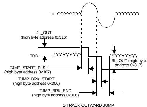
Figure 13 Single-Track Outward Jumping
