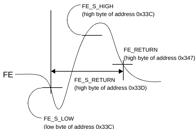
Figure 20 Focus Error S-Curve
