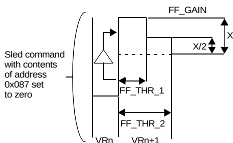
Figure 18 Applying Feed-Forward Correction
