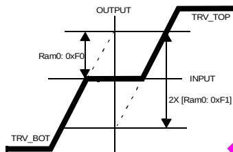
Figure 12 Sled Dead Band Parameters
