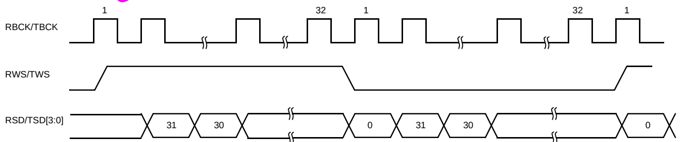
Figure 33 Right Justified Mode / 32-Bit Cycle Frame / 24-Bit Data Frame / LSB First
