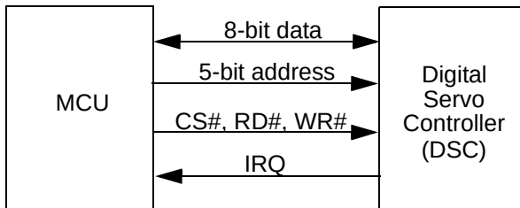
Figure 5 Servo Controller / MCU Interface
