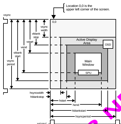
Figure 26 Video Output Timing
