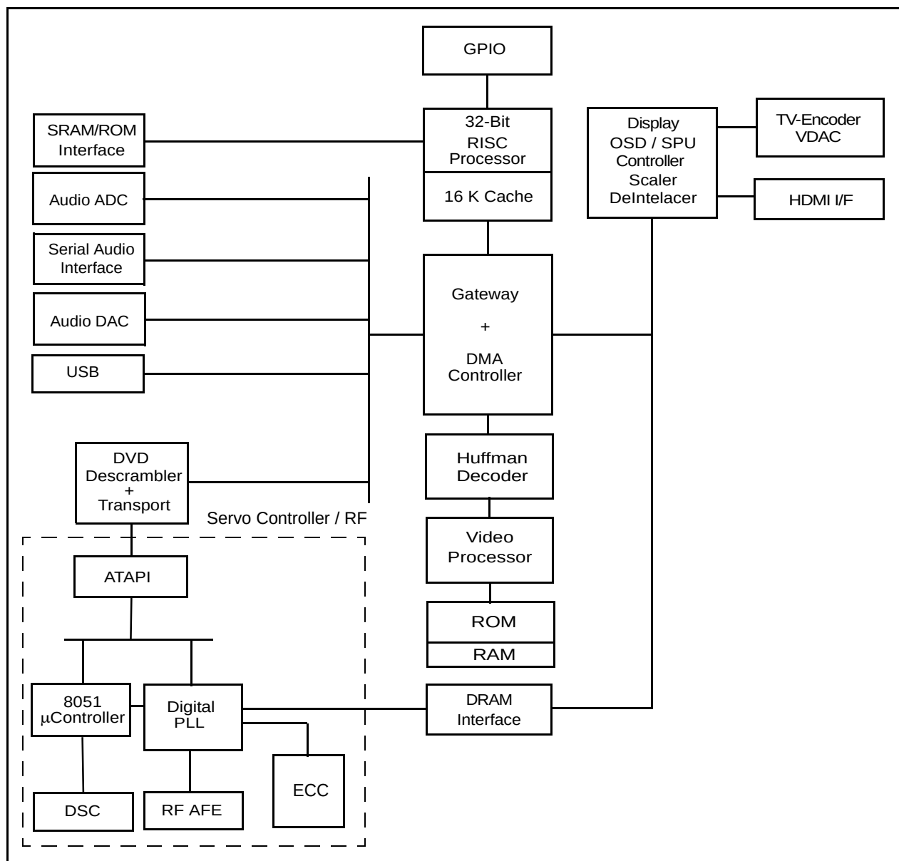
Figure 3 ES8381 Phoenix Block Diagram
