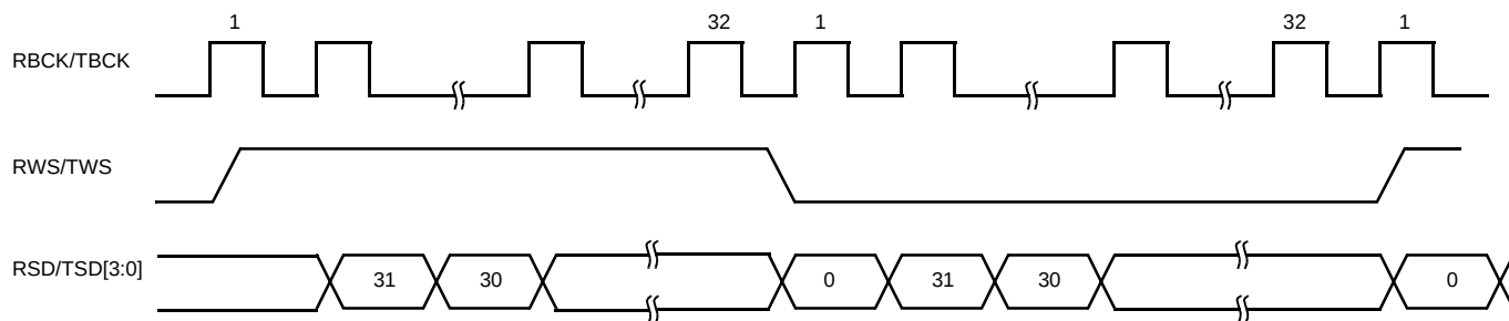
Figure 34 Left Justified Mode / 32-Bit Cycle Frame / 24-Bit Data Frame / MSB First
