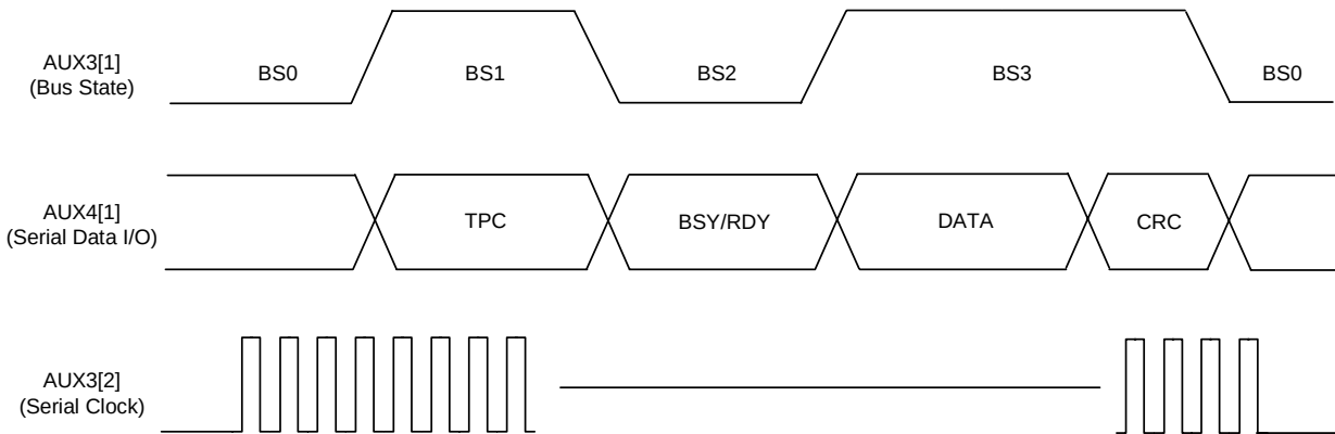
Figure 40 Memory Stick Read Timing
