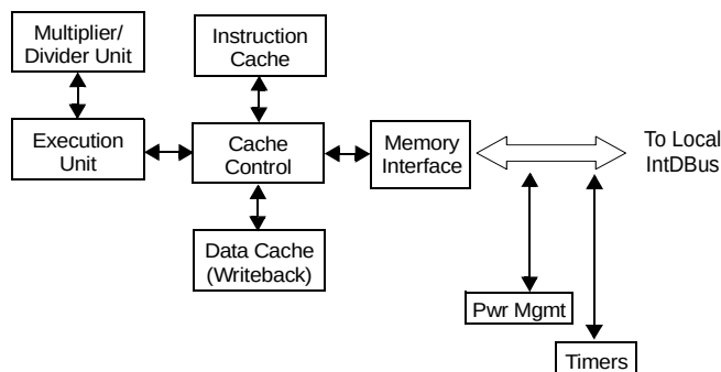
Figure 23 ESS RISC Block Diagram
