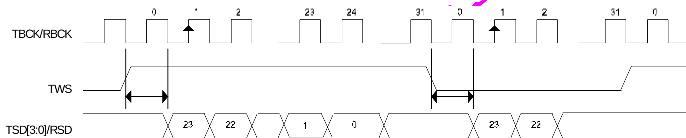
Figure 35 I²S Mode
