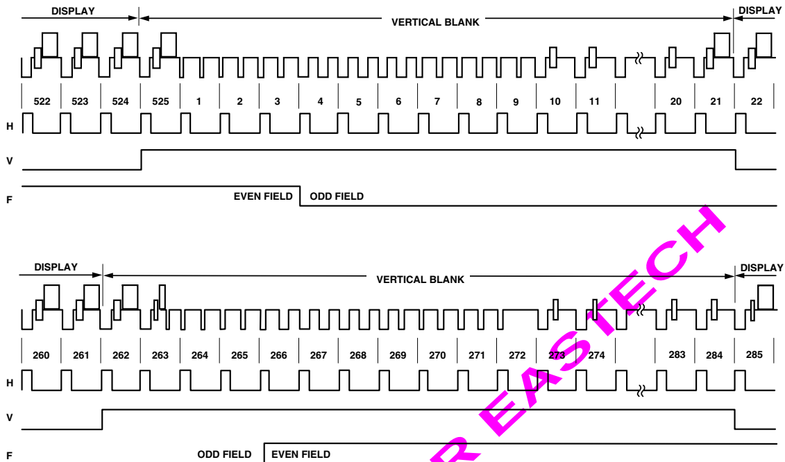
Figure 51 NTSC Timing
