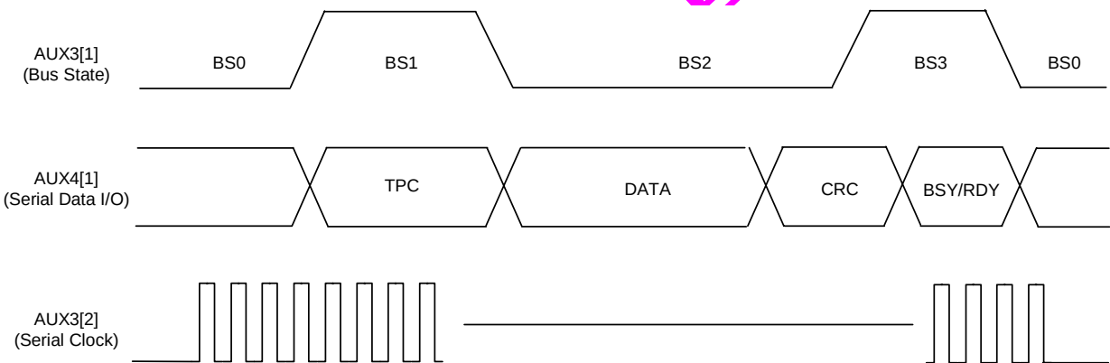
Figure 41 Memory Stick Write Timing
