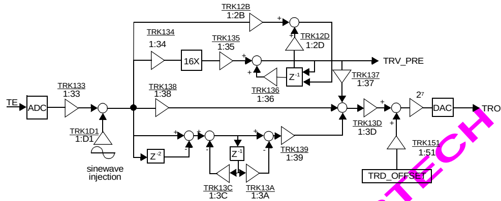
Figure 10 Tracking Equalizer During Playback
