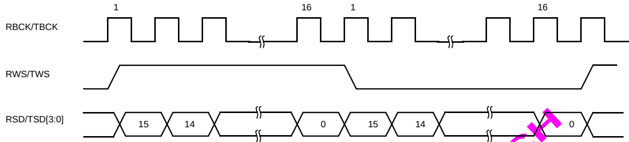
Figure 31 Right Justified Mode / 16-Bit Cycle Frame / 16-Bit Data Frame / MSB First
