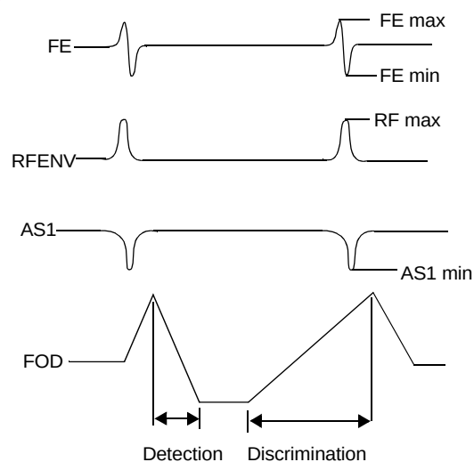
Figure 21 Detection and Discrimination Timing Diagrams
