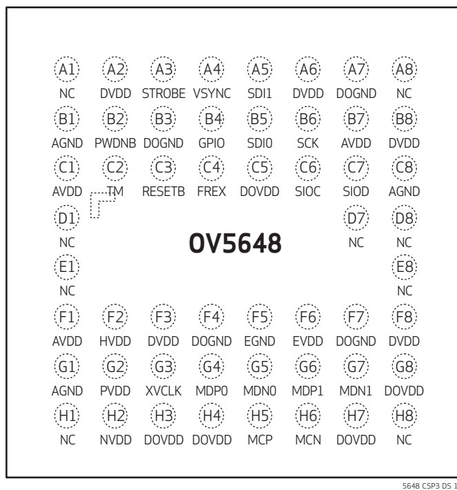
figure 1-1 pin diagram
