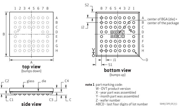
figure 9-1 package specifications
