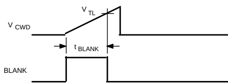
Normal commutation
