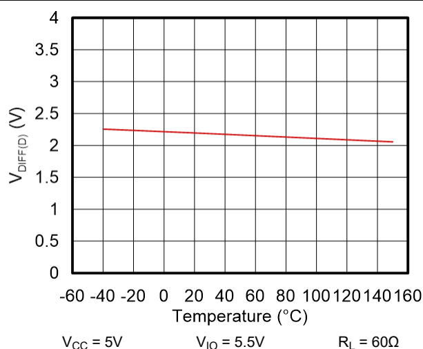
Figure 5-2. V_{DIFF(D)} vs. Temperature
