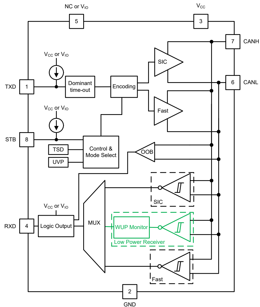
Figure 7-3. Block Diagram
