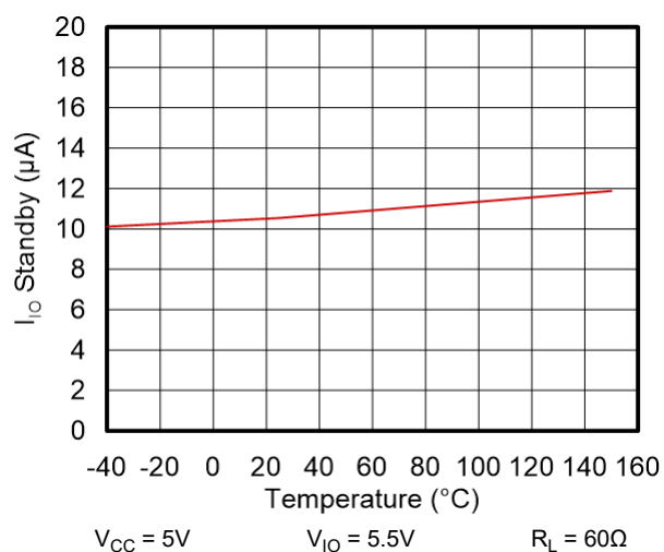
I_{IO} Standby vs. Temperature
