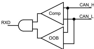
Figure 7-12. OOB Comparator Output to RXD
