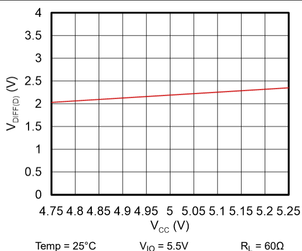
Figure 5-3. V_{DIFF(D)} vs. V_{CC}
