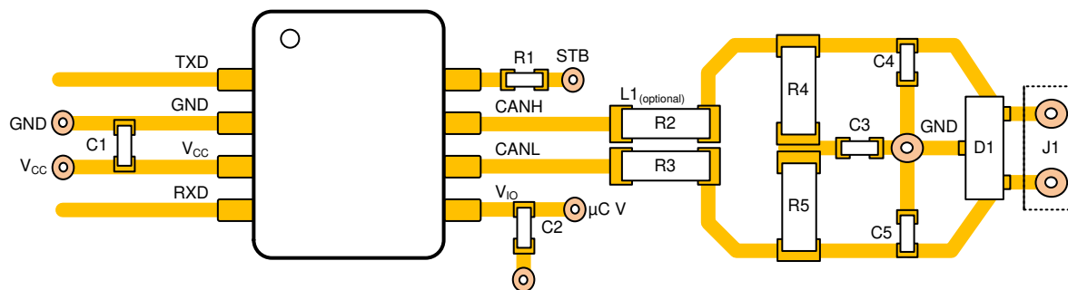
Figure 8-6. Layout Example
