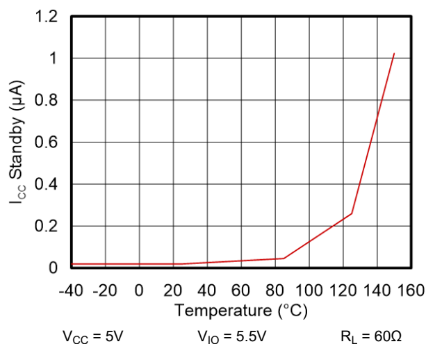
Figure 5-1. I_{CC} Standby vs. Temperature
