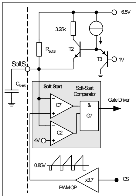
Figure 7 Soft Start
