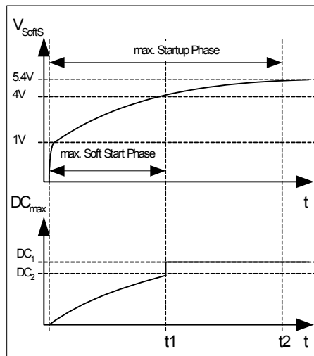
Figure 8 Startup Phase
