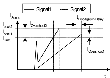
Figure 14 Current Limiting
