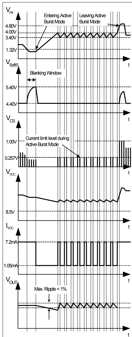
Figure 19 Signals in Active Burst Mode
