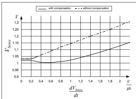
Figure 15 Overcurrent Shutdown
