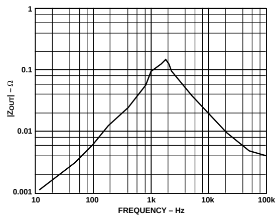
Figure 9. Incremental Output Impedance (Magnitude)
