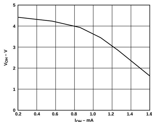
Figure 32. Source Capability of Status Output
