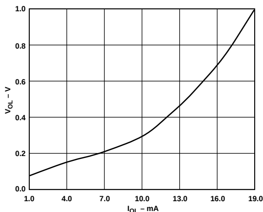
Figure 33. Sink Capability of Status Output
