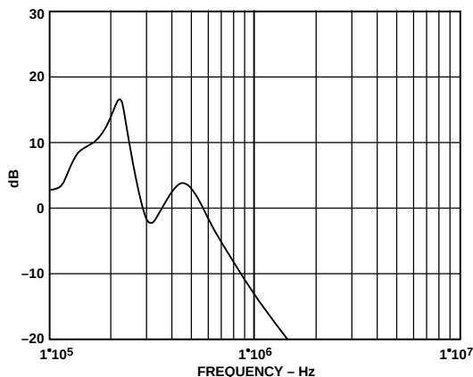
Figure 41. Change in ADDC02808PB Differential Emissions vs. the ADDC02805SA Emissions with External 0.5 \mu H, 16 A Inductor
