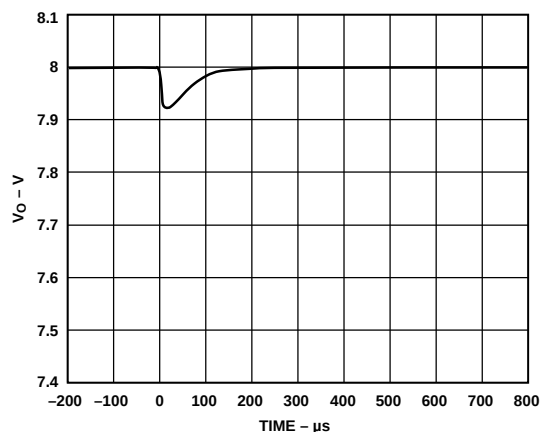
Figure 25. Predicted Response for 24 A Step Load Change, di/dt = 12 \text{ A}/\mu\text{s} , with Factory Set Internal Compensation Optimized for C_{\text{LOAD}} = 4,000 \mu\text{F} and R_{\text{ESR}} = 2.5 \text{ m}\Omega
