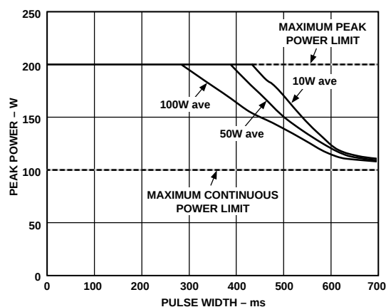
Figure 16. Largest On-State Power vs. Pulse Width that Maintains T_{JMAX} \leq 110^\circ\text{C} at 25^\circ\text{C} Baseplate
