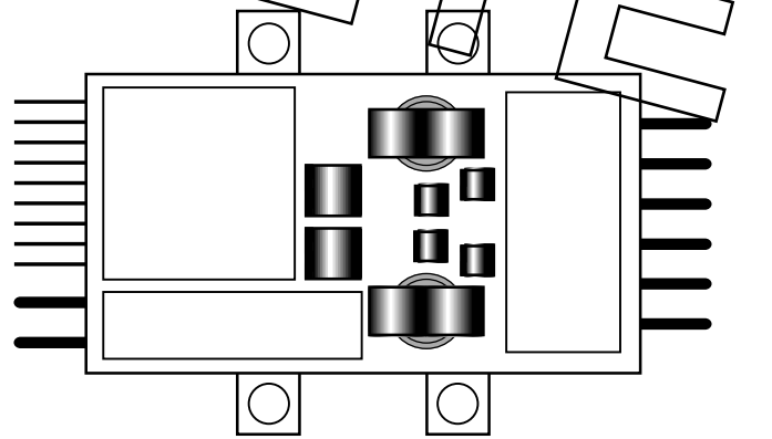
Figure 24. Hot Spots (Shaded Areas) of DC/DC Converter
