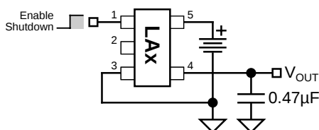
Regulator Circuit
