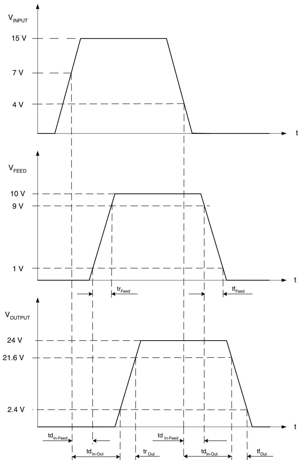
Figure 7-1. Timing Diagram (1) 1
