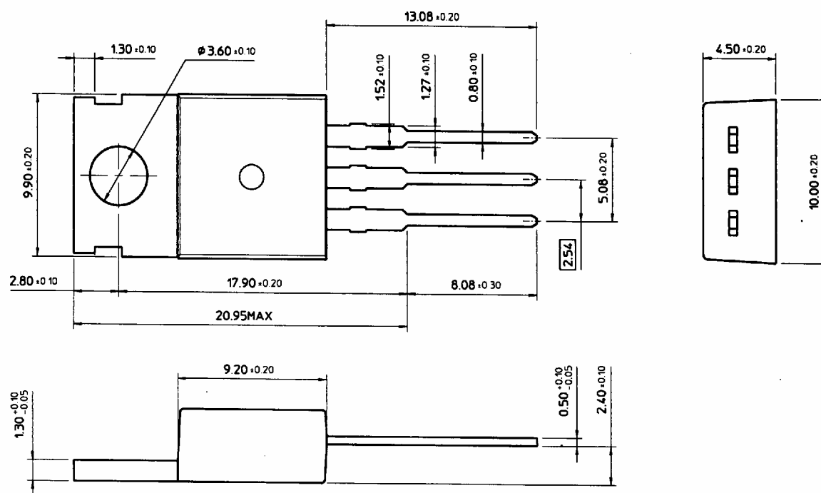
TO-220 (1)
