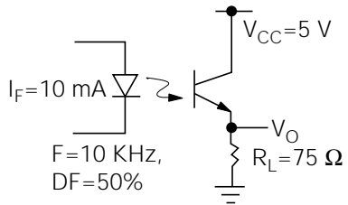
Figure 10. Switching schematic
