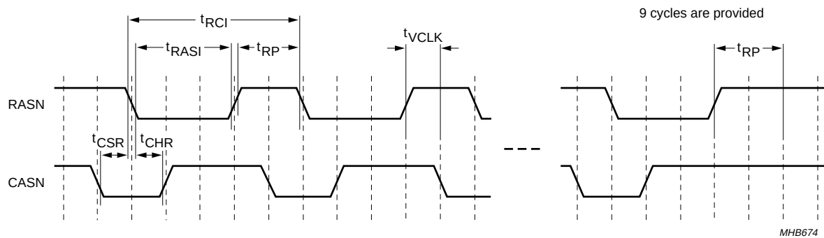
Fig.15 DRAM initialization sequence.
