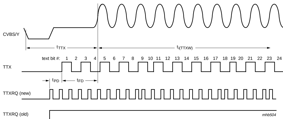
Fig 23. Teletext timing
