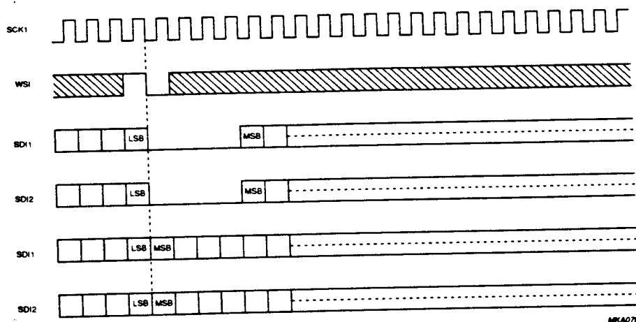
Fig.6 Simultaneous mode input format - continuous clock idling on MSB.
