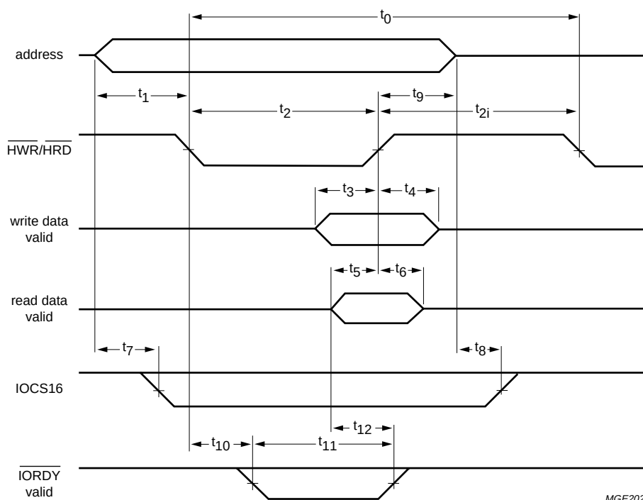
Fig.14 PIO 8 and 16-bit transfer.
