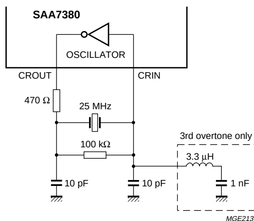
Fig.25 Crystal oscillator circuit.
