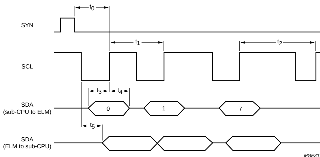
Fig.13 Sub-CPU interface timing diagram.
