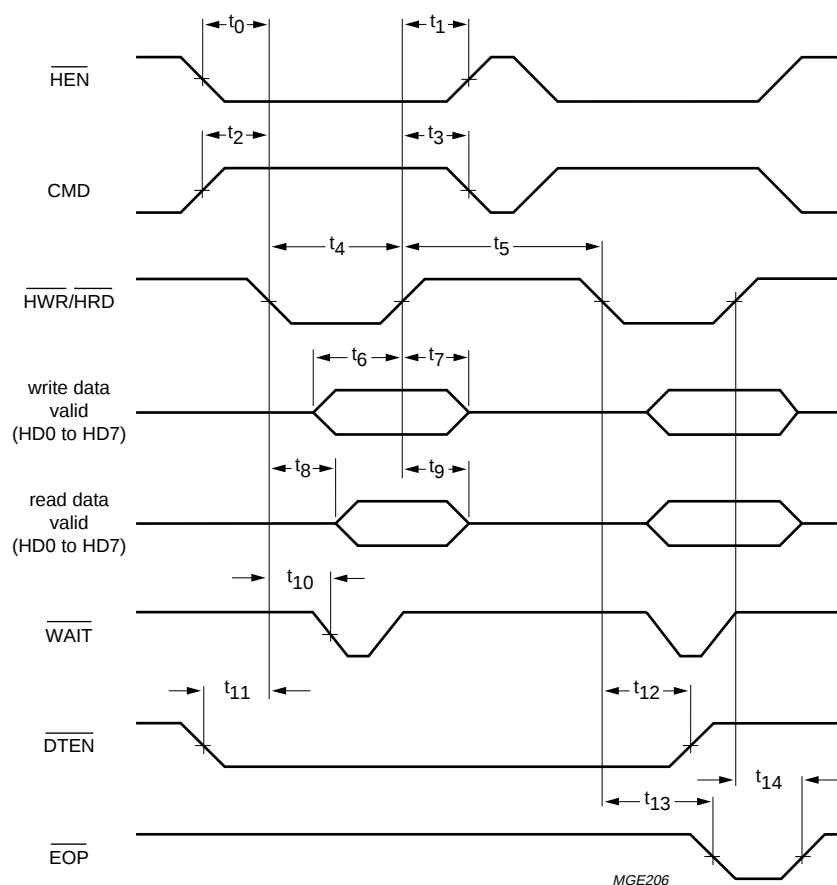
Fig.18 WAIT control and data transfer.
