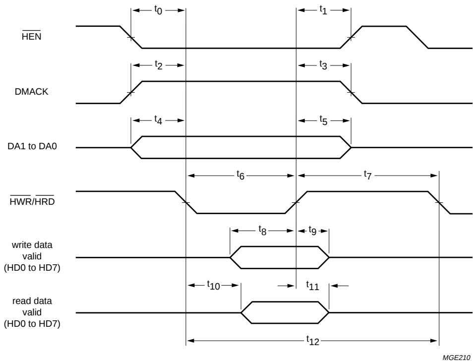
Fig.22 Non-DMA data transfer.
