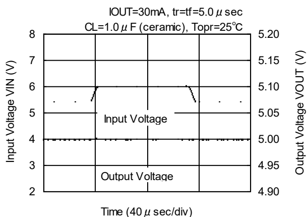
XC6403/04 Series (VR: 5.0V)
