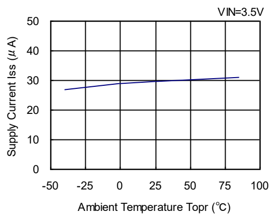
XC6403/04 Series (VR: 2.5V)
