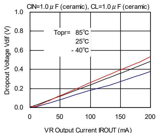
XC6403/04 Series (VR: 5.0V)
