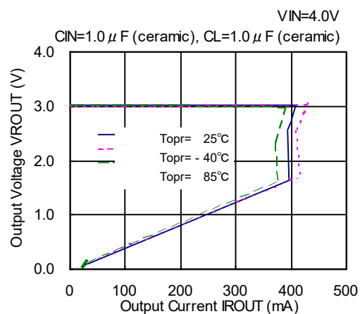
XC6403 Series (VR: 3.0V)
