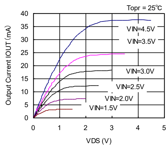
XC6403/04 Series (VD: 5.0V)
