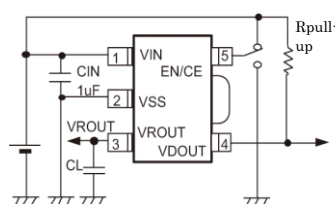
XC6404 A, C, D Series
