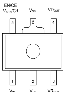
SOT-89-5 (TOP VIEW)
