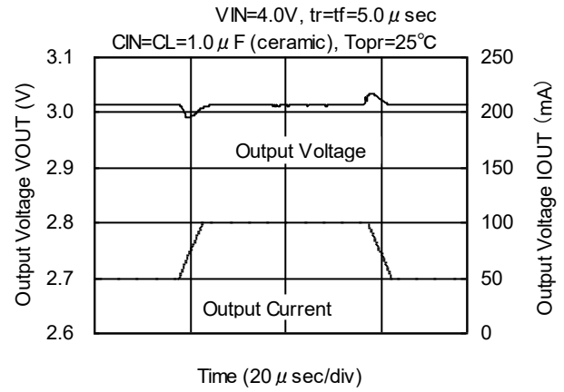
XC6403/04 Series (VR: 3.0V)
