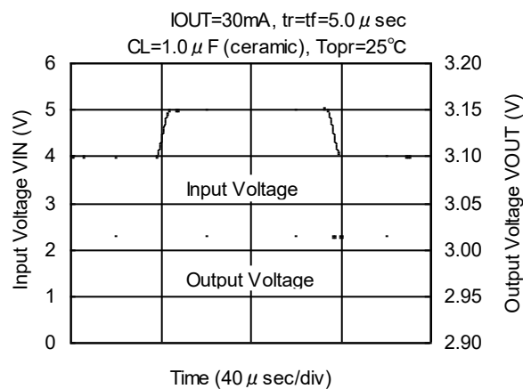
XC6403/04 Series (VR: 3.0V)
