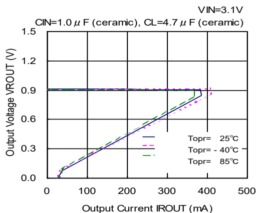
XC6403 Series (VR: 0.9V)
