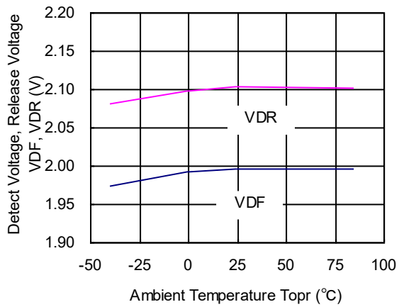
XC6403/04 Series (VD: 2.0V)
