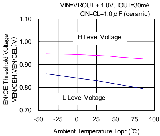
(7) EN/CE Threshold Voltage vs. Ambient Temperature
