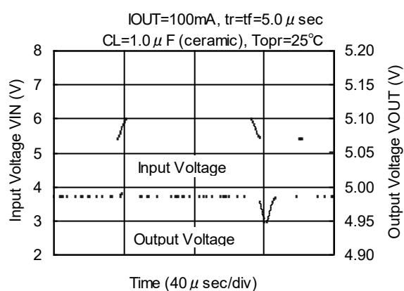
XC6403/04 Series (VR: 5.0V)
