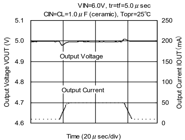
XC6403/04 Series (VR: 5.0V)
