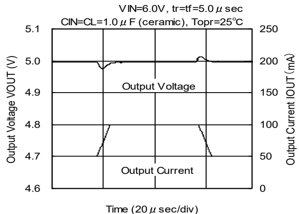
XC6403/04 Series (VR: 5.0V)
