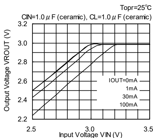
XC6403/04 Series (VR: 3.0V)
