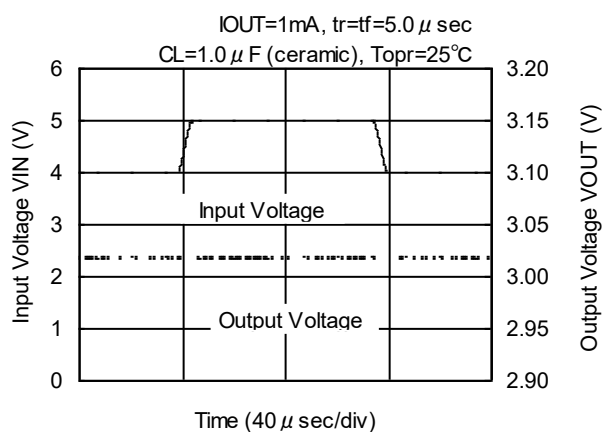
XC6403/04 Series (VR: 3.0V)
