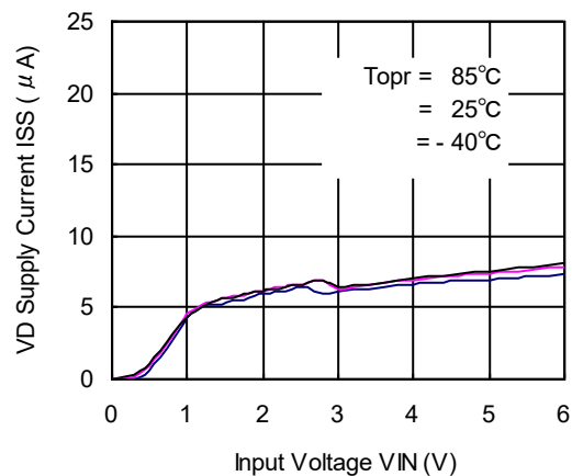
XC6403/04 Series (VD: 2.7V)
