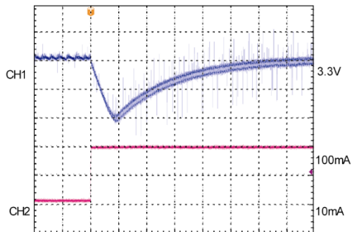
200 \mu sec/div CH1: V_{OUT1,2} , AC-COUPLED, 50mV/div CH2: I_{OUT1,2} , 50mA/div
