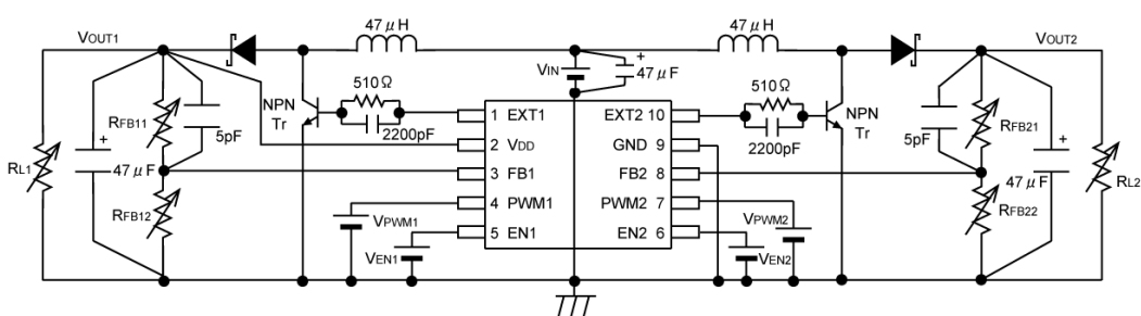
Circuit 3
