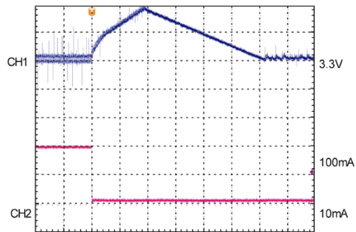
200 \mu sec/div CH1: V_{OUT1,2} , AC-COUPLED, 50mV/div CH2: I_{OUT1,2} , 50mA/div
