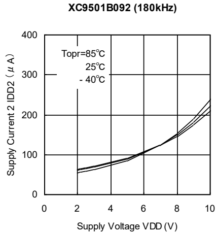
(7) Supply Current 2 vs. Supply Voltage
