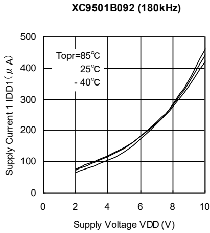
(4) Supply Current vs. Supply Voltage
