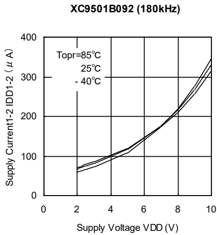
(6) Supply Current 1-2 vs. Supply Voltage
