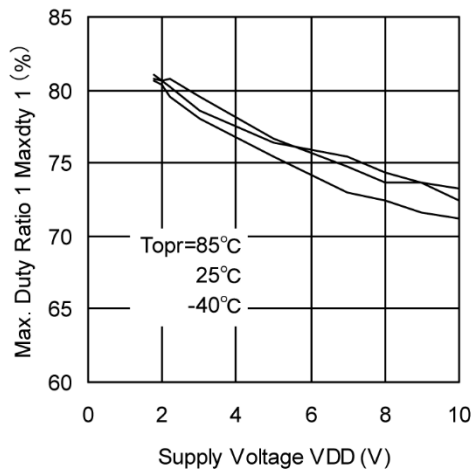
(17) Maximum Duty Ratio 1 vs. Supply Voltage
