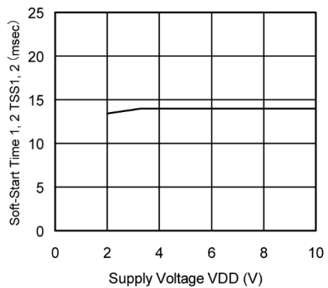
XC9502B092 (180kHz)
