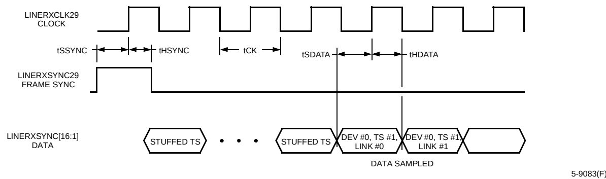
Figure 13. Parallel System Bus Interface Receive I/O Timing
