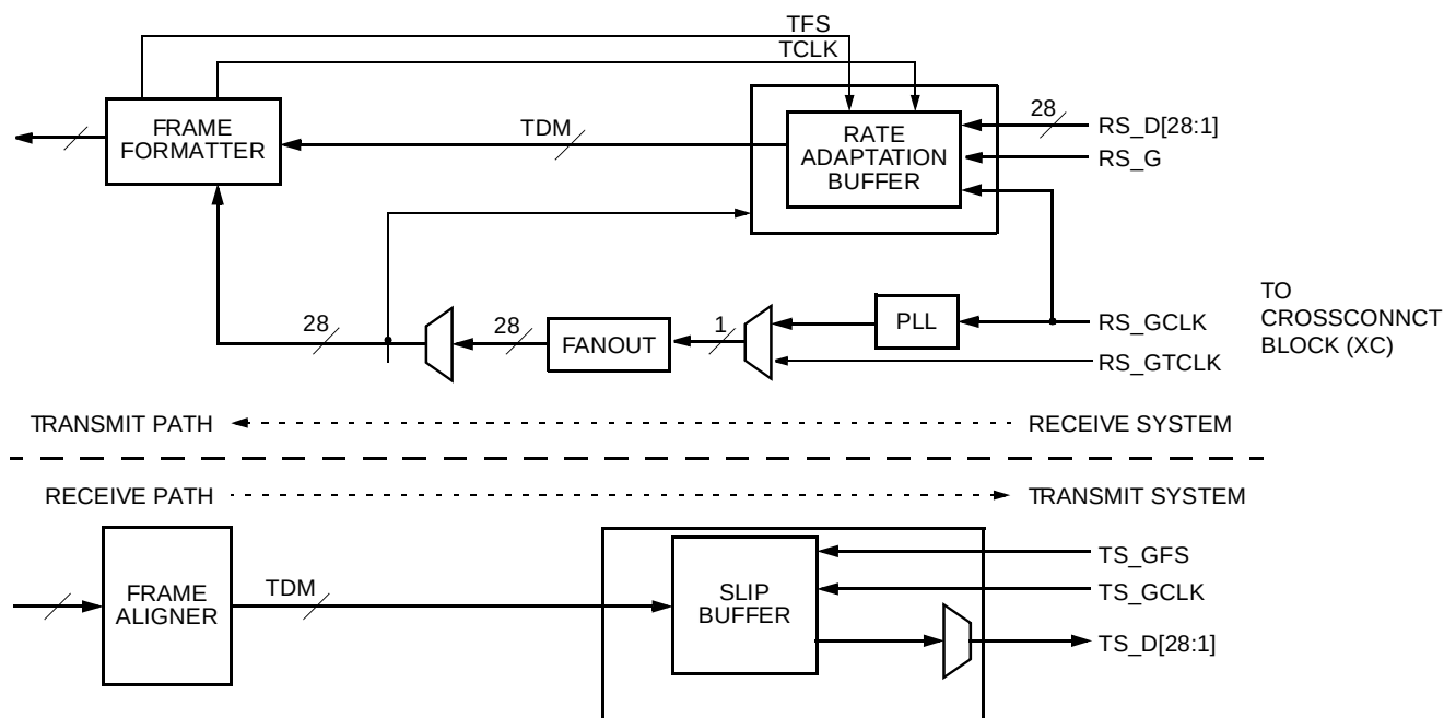
Figure 69. CHI Mode of the Transmit System Interface
