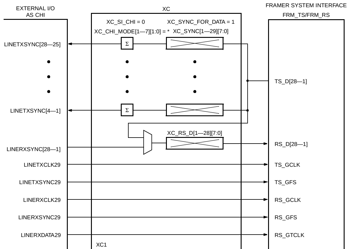
Figure 87. Framers System Interface—Concentration Highway Interface (CHI)
