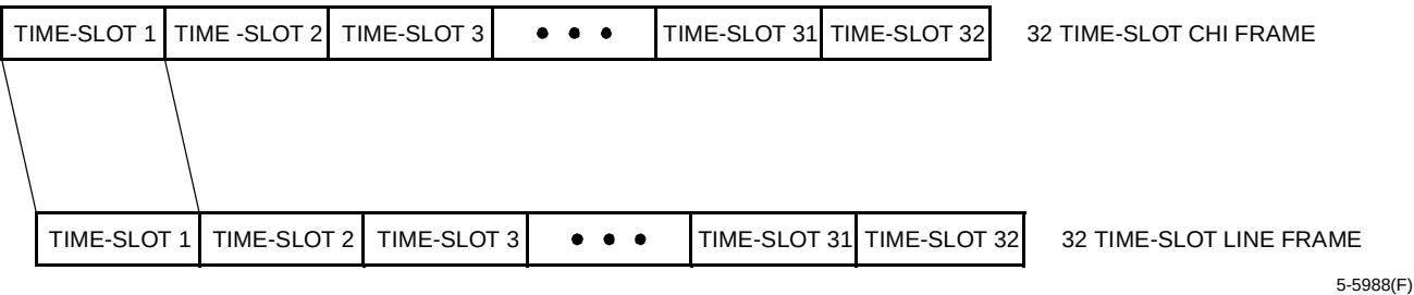
Figure 59. CEPT Transparent Frame Structure
