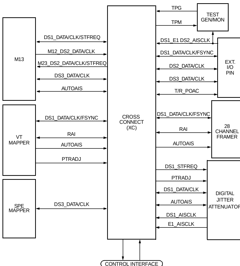
Figure 81. Cross Connect Block Diagram
