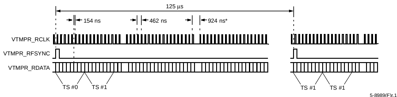
Figure 44. E1 Interface
