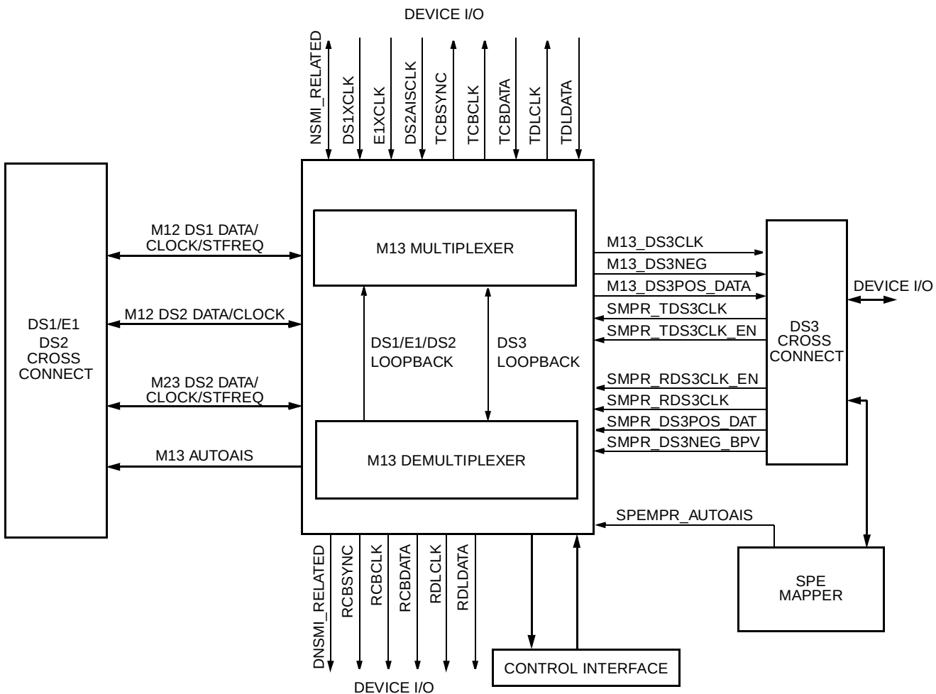
Figure 47. M13 Block Diagram
