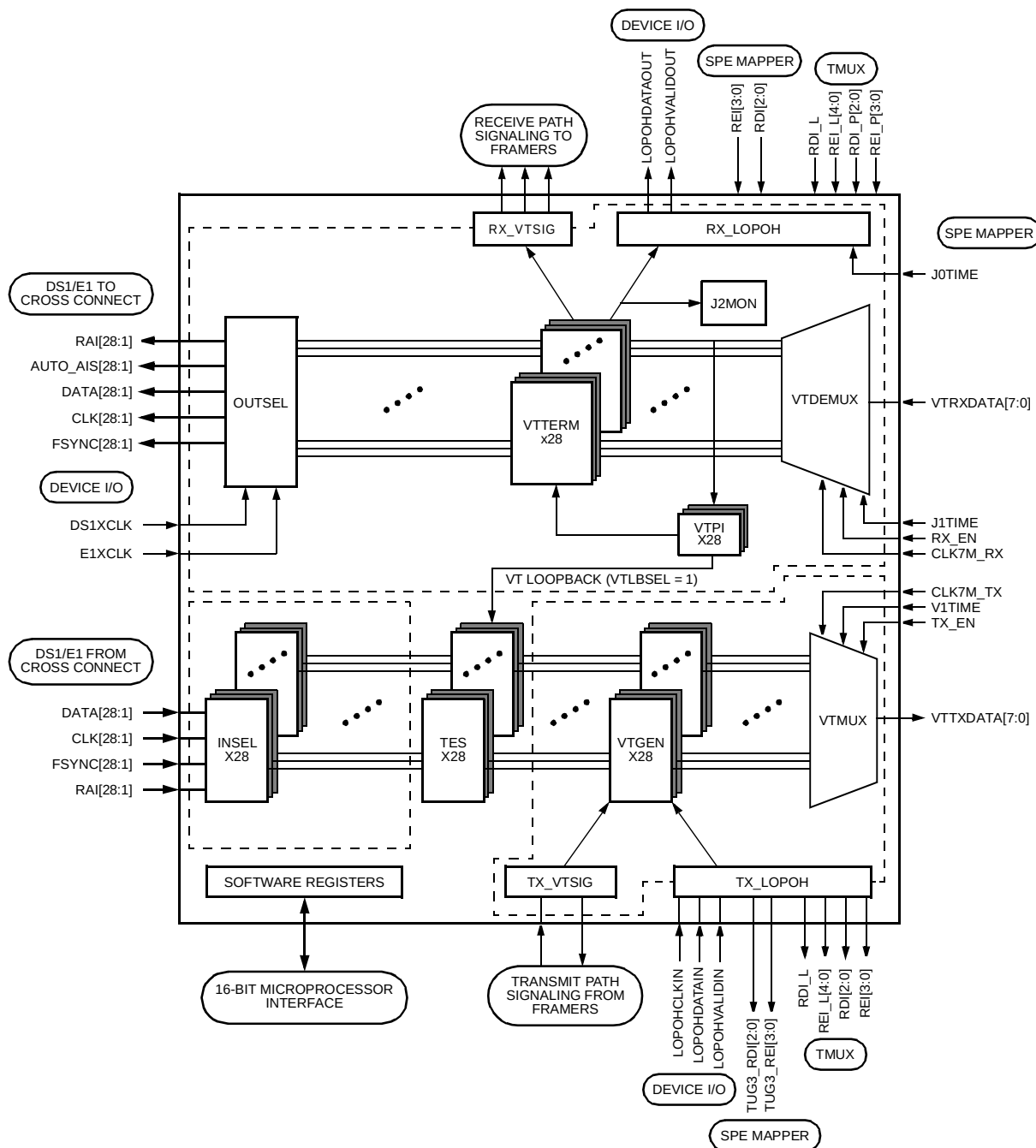
Figure 39. VT Mapper Functional Block Diagram
