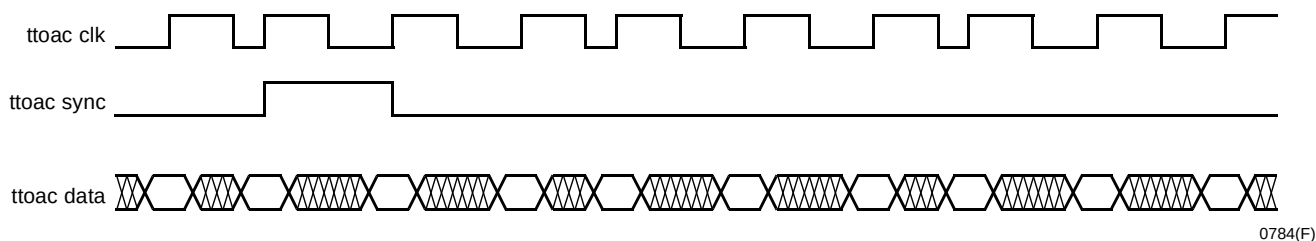
Figure 22. TMUX TTOAC and RTOAC Timing Diagram
