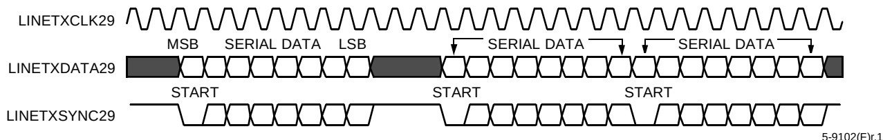
Figure 80. Network Serial Multiplexed Interface (Multiple Octets)
