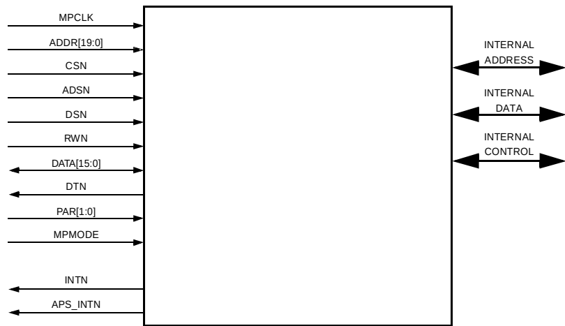
Figure 18. Microprocessor Interface
