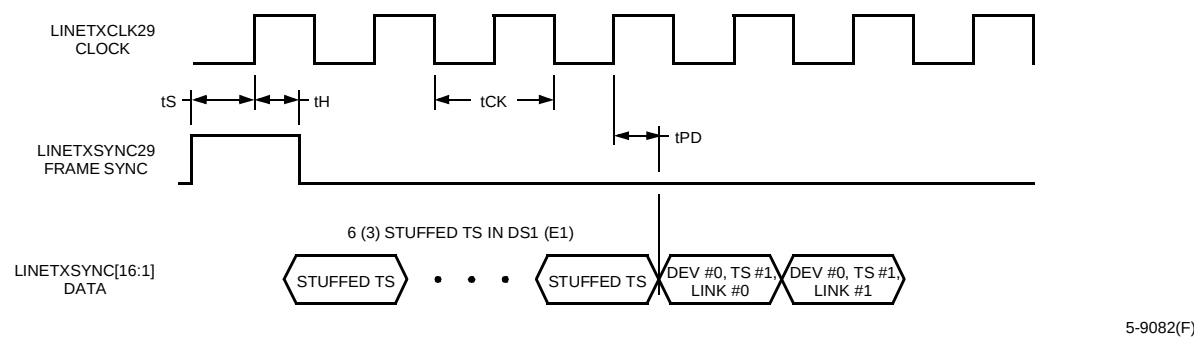
Figure 12. Parallel System Bus Interface Transmit I/O Timing
