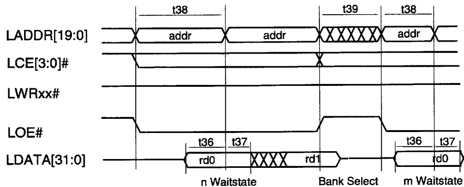
Figure 15. SRAM Read Timing
