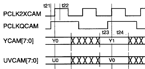
Figure 5. 2x Clock Mode Video In Bus Timing
