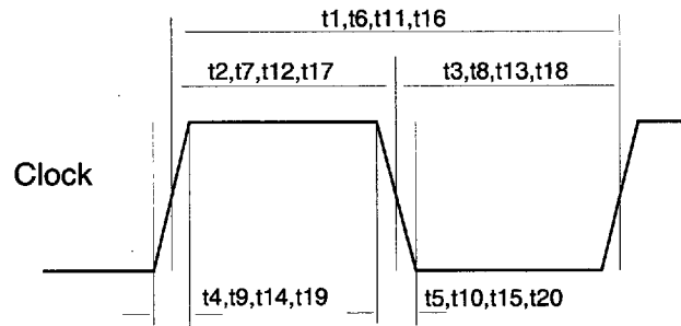
Figure 25. Clock Timing Diagram
