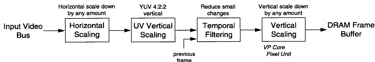
Figure 3. Video Pre-processing
