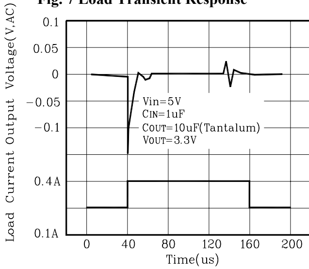
Fig. 7 Load Transient Response
