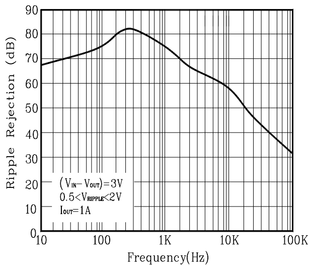
Fig. 9 Ripple Rejection
