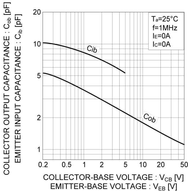
Fig.21 Collector Output Capacitance vs. ollector-Base Voltage Emitter Input Capacitance vs. Emitter-Base Voltage
