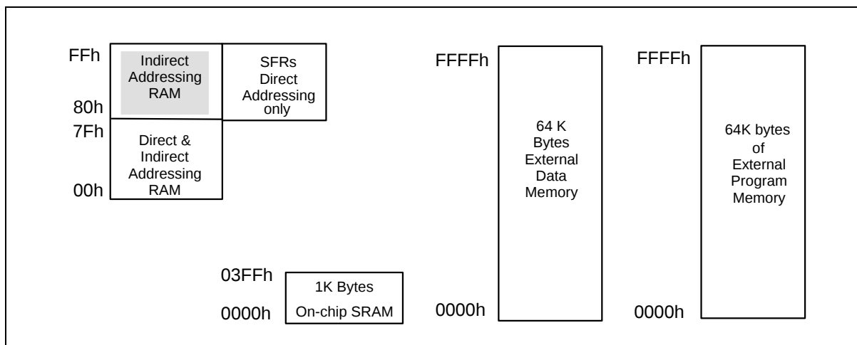
Figure 1. Memory Map
