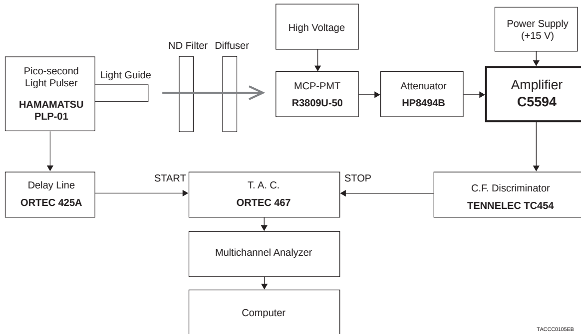
Figure 4: Measurement Set-up
