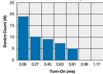
IBB110P Typical Turn-On Time (N=50 Ambient Temperature = 25°C) (Load Current = 100mADC; I_F = 5\text{mAADC} )
