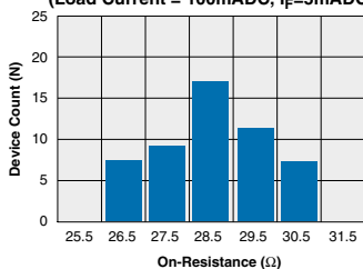
IBB110P Typical On-Resistance Distribution (N=50 Ambient Temperature = 25°C) (Load Current = 100mADC, I_F = 5\text{mAADC} )
