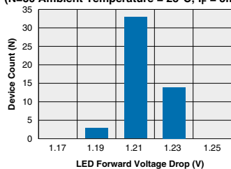
IBB110P Typical LED Forward Voltage Drop (N=50 Ambient Temperature = 25°C; I_F = 5\text{mAADC} )
