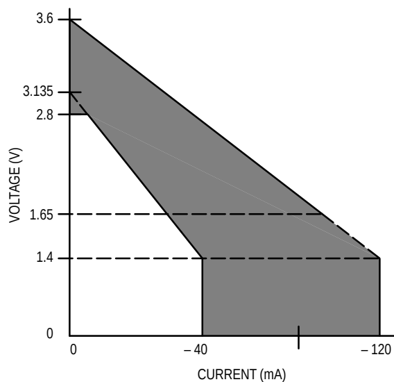
(a) Pull-Up for 3.3 V I/O Supply
