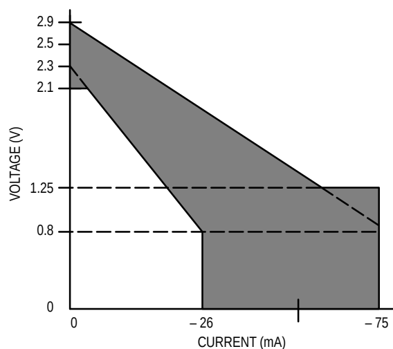
(b) Pull-Up for 2.5 V I/O Supply
