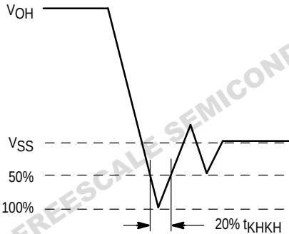
Figure 2. Undershoot Voltage
