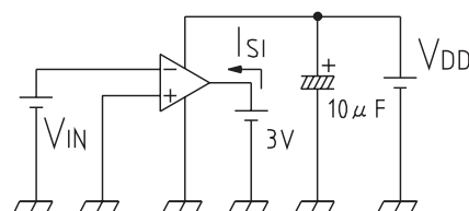
■ Measuring circuit 10
