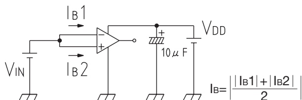
■ Measuring circuit 2
