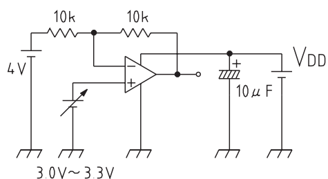
■ Measuring circuit 5
